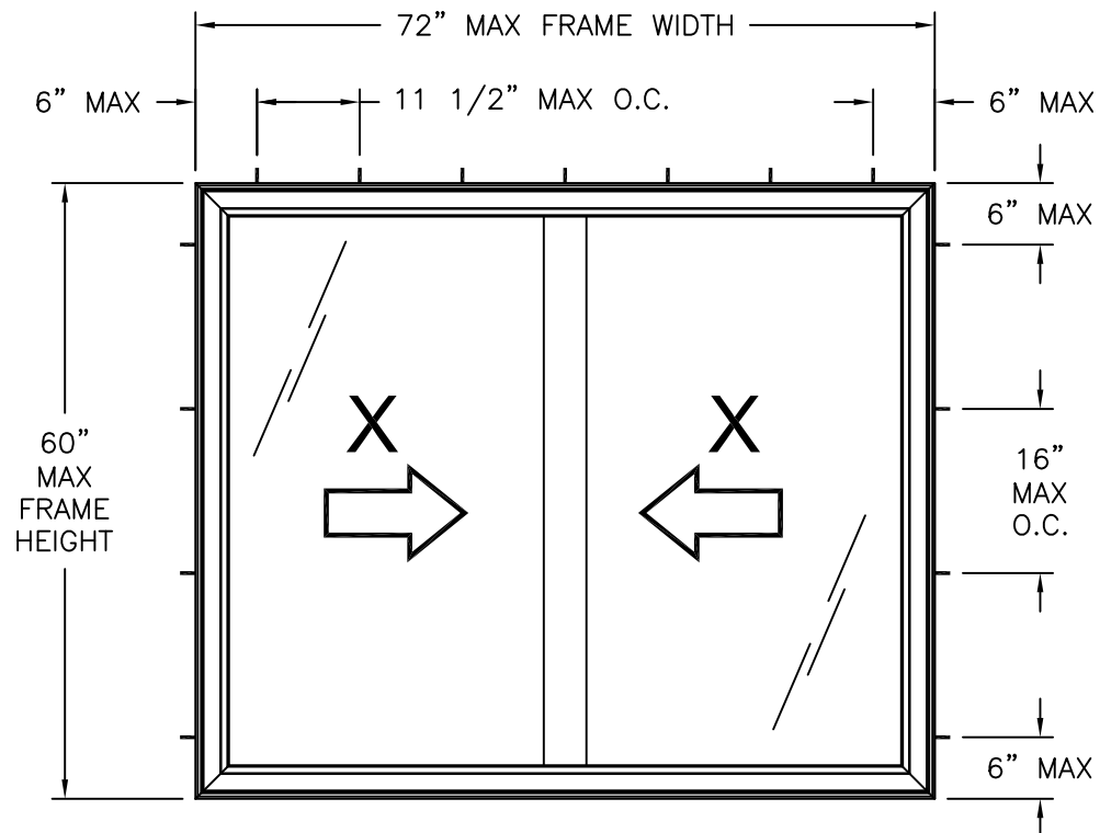
SIGNATURE/CAMBRIDGE HORIZONTAL SLIDER XX EXTERIOR VIEW FRAME INSTALLATION
