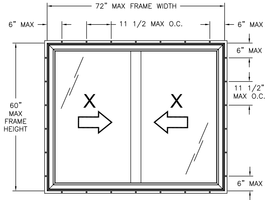
SIGNATURE/CAMBRIDGE HORIZONTAL SLIDER XX EXTERIOR VIEW FIN INSTALLATION
