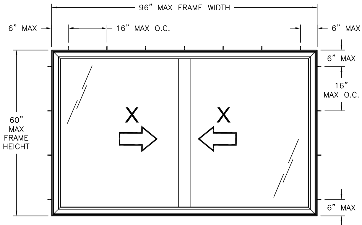
SIGNATURE/VIWINCO HORIZONTAL SLIDER XX EXTERIOR VIEW FRAME INSTALLATION
