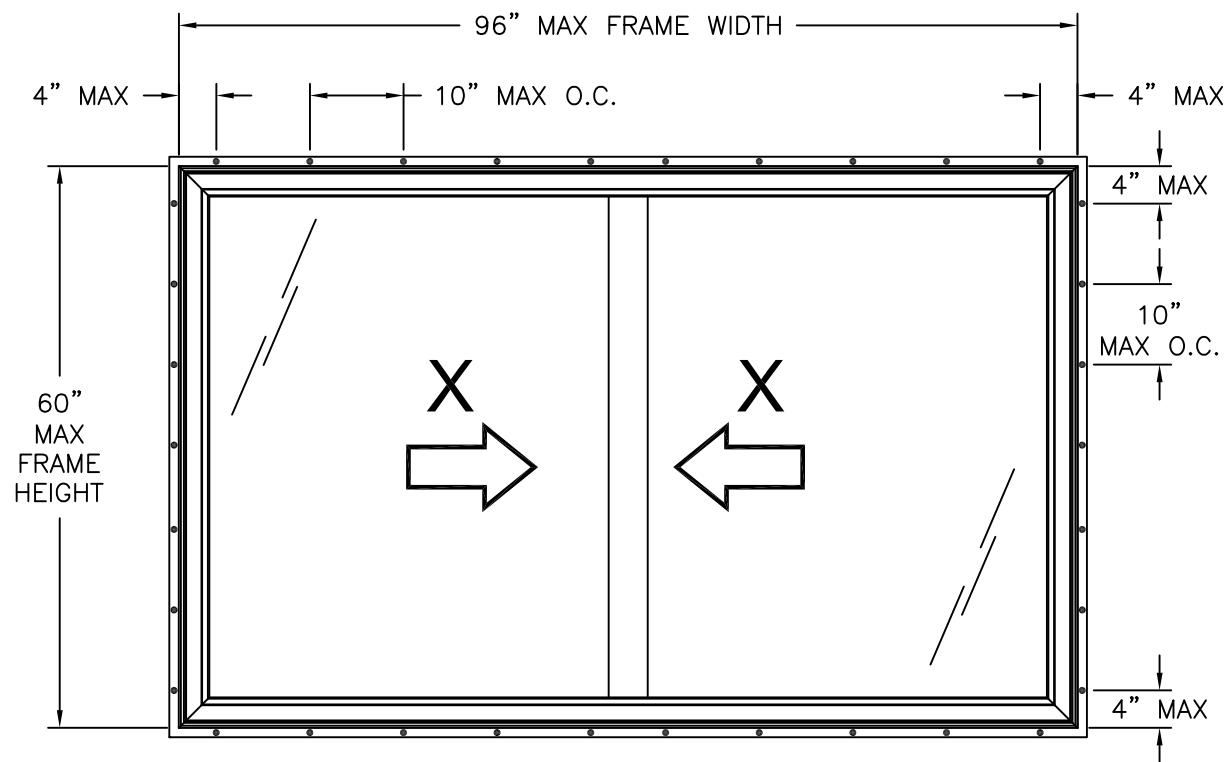
SIGNATURE/VIWINCO HORIZONTAL SLIDER XX EXTERIOR VIEW FIN INSTALLATION
