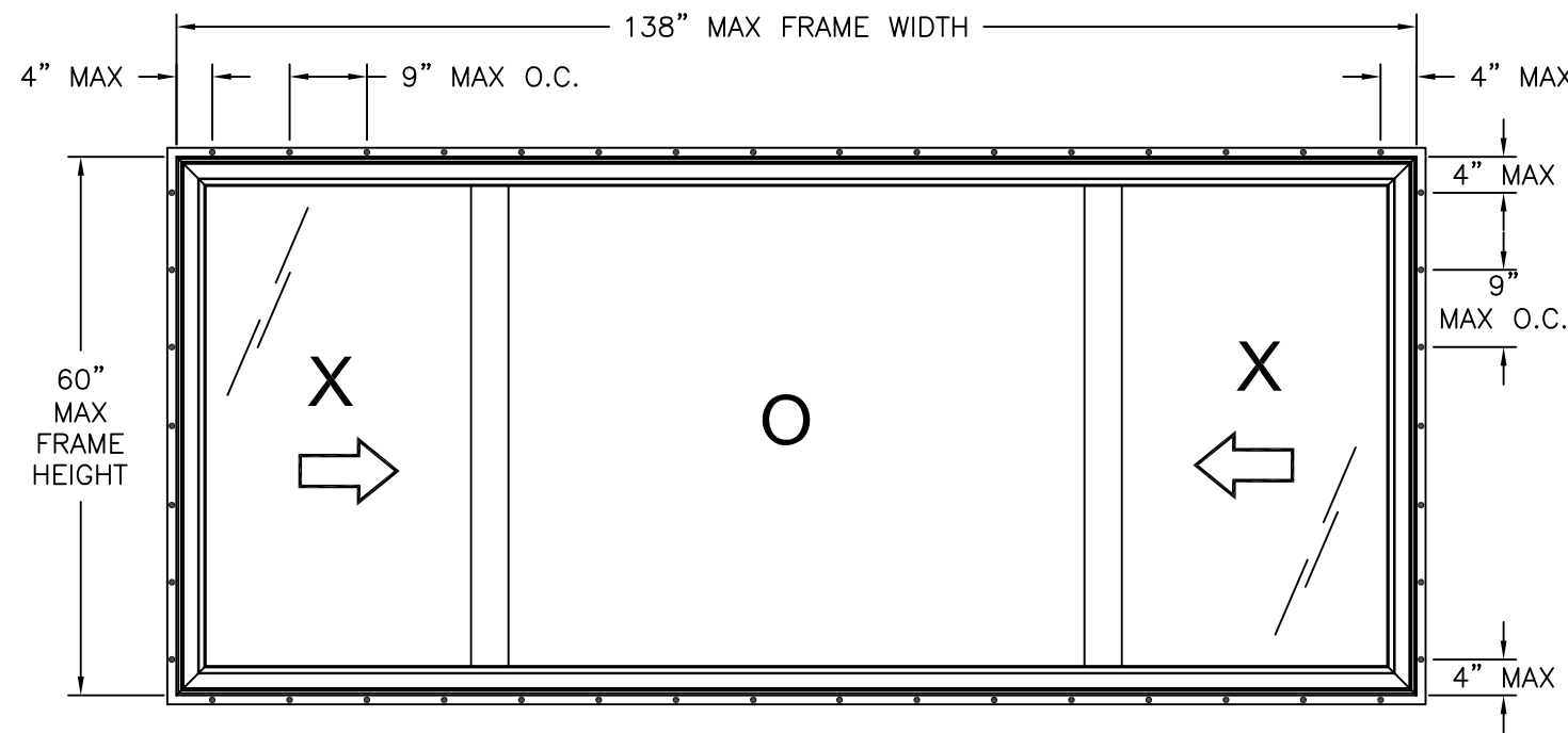
SIGNATURE/VIWINCO HORIZONTAL SLIDER XOX EXTERIOR VIEW FIN INSTALLATION
