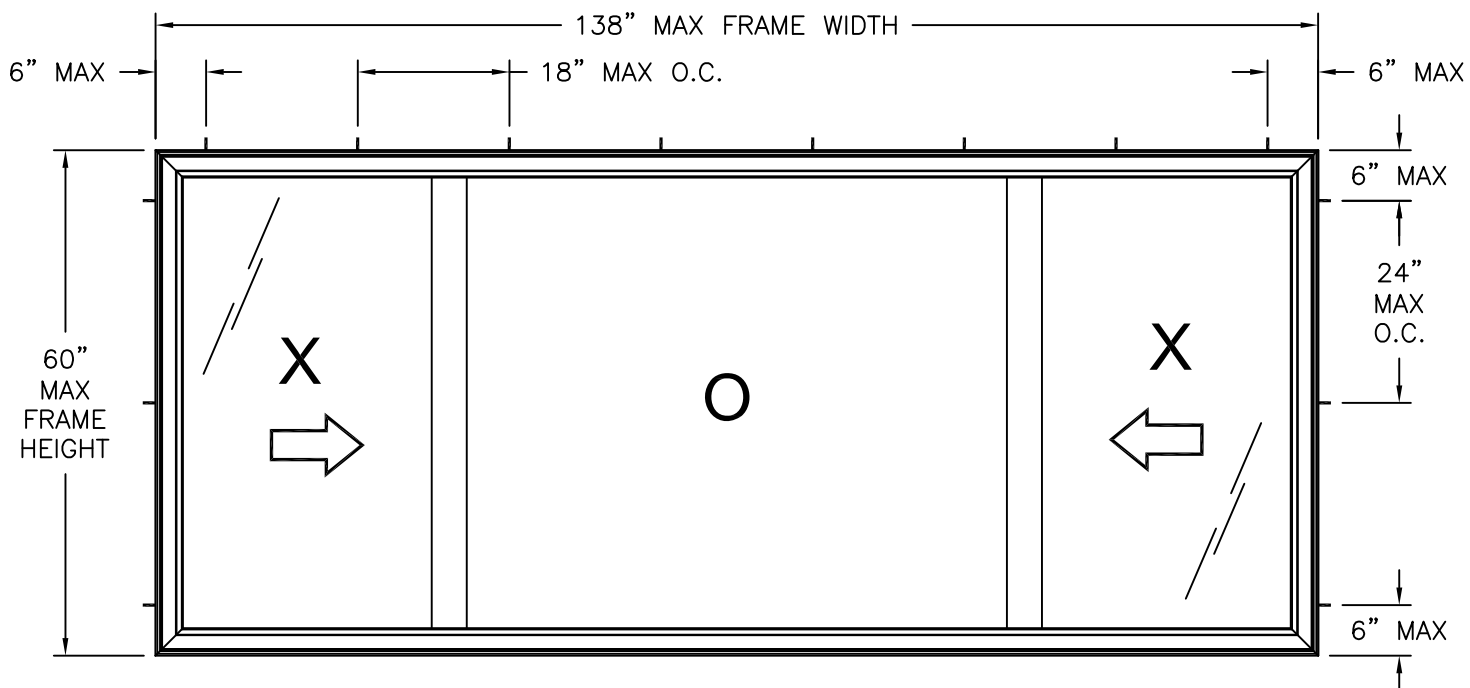
SIGNATURE/VIWINCO HORIZONTAL SLIDER XOX EXTERIOR VIEW FRAME INSTALLATION
