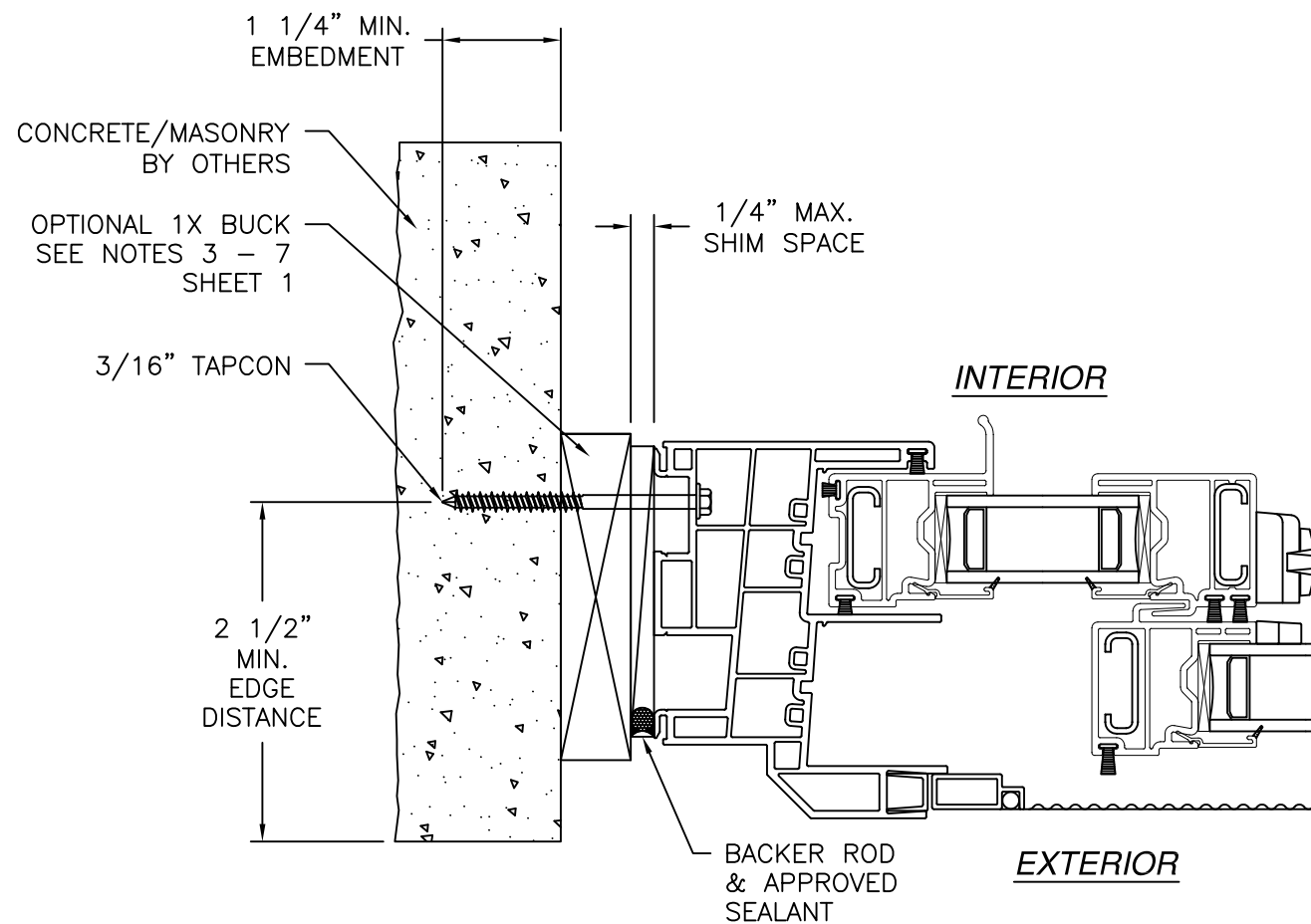
JAMB INSTALLATION DETAIL CONCRETE/MASONRY INSTALLATION
