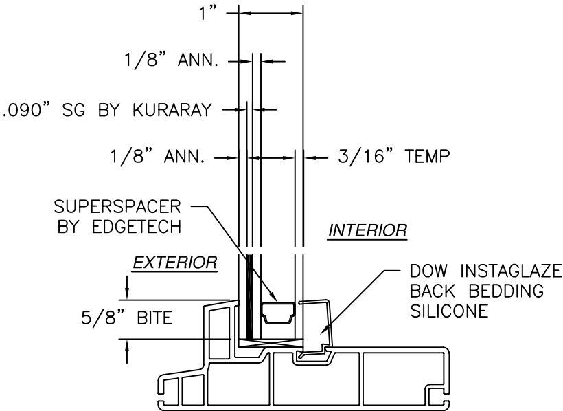
GLAZING DETAIL
