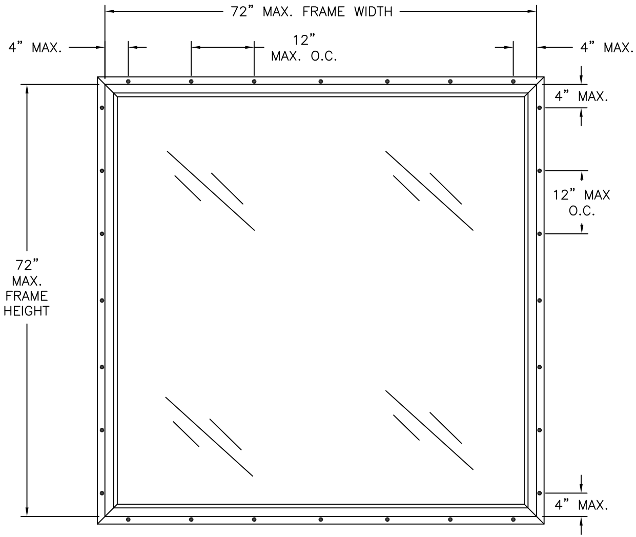
OCEANVIEW GEOMETRIC IMPACT PICTURE EXTERIOR VIEW FIN INSTALLATION
