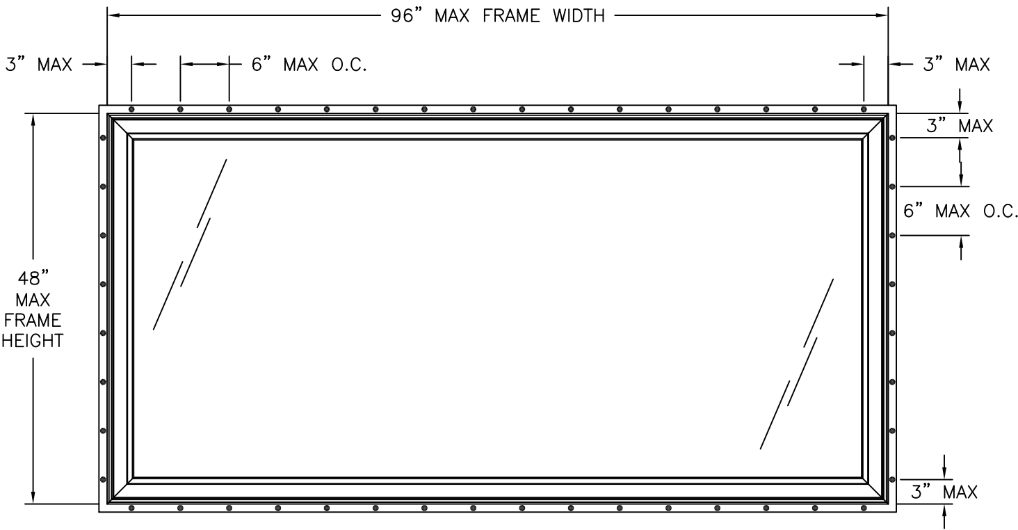
S-SERIES TRANSOM EXTERIOR VIEW FIN INSTALLATION
