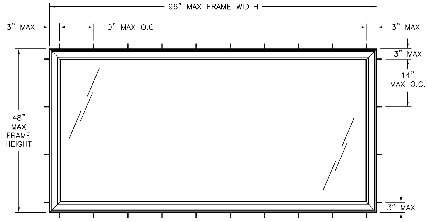
CAMBRIDGE TRANSOM EXTERIOR VIEW FRAME INSTALLATION
