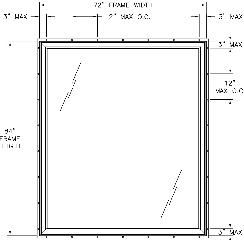
S-SERIES GEO FIXED EXTERIOR VIEW FIN INSTALLATION
