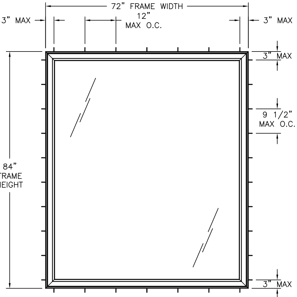
CAMBRIDGE GEO FIXED EXTERIOR VIEW FRAME INSTALLATION
