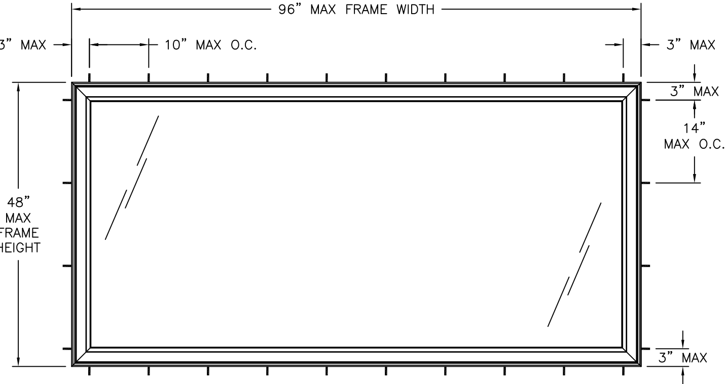
CAMBRIDGE GEOMETRIC EXTERIOR VIEW FRAME INSTALLATION
