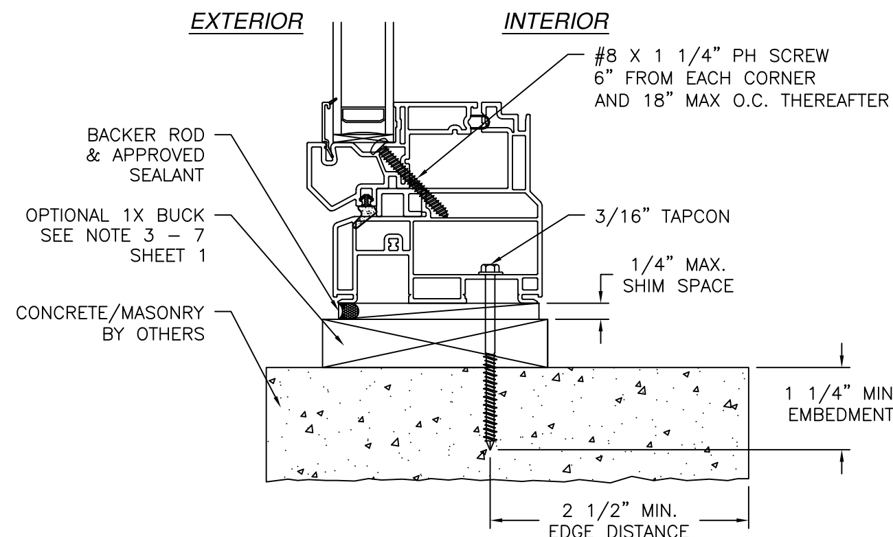
VERTICAL CROSS SECTION CONCRETE/MASONRY INSTALLATION
