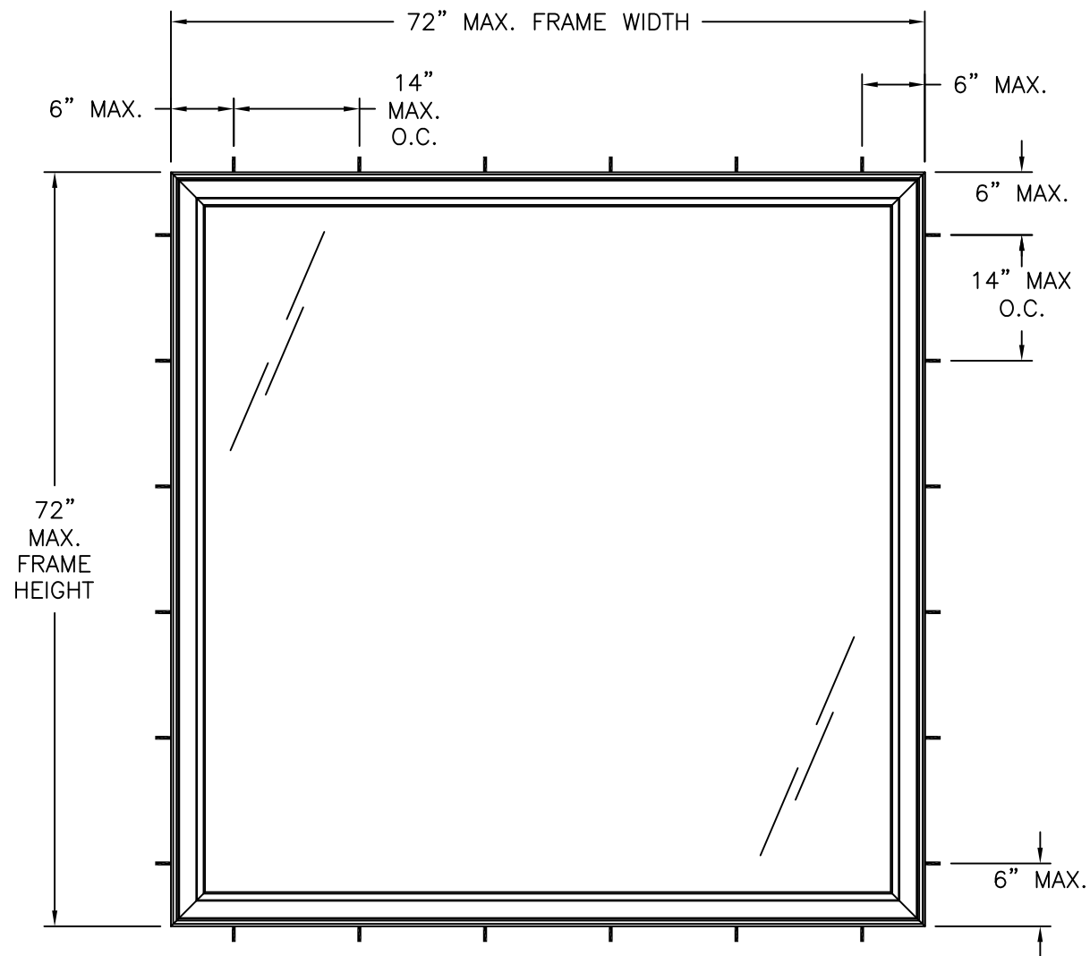
CAMBRIDGE CASEMENT PICTURE EXTERIOR VIEW FRAME INSTALLATION
