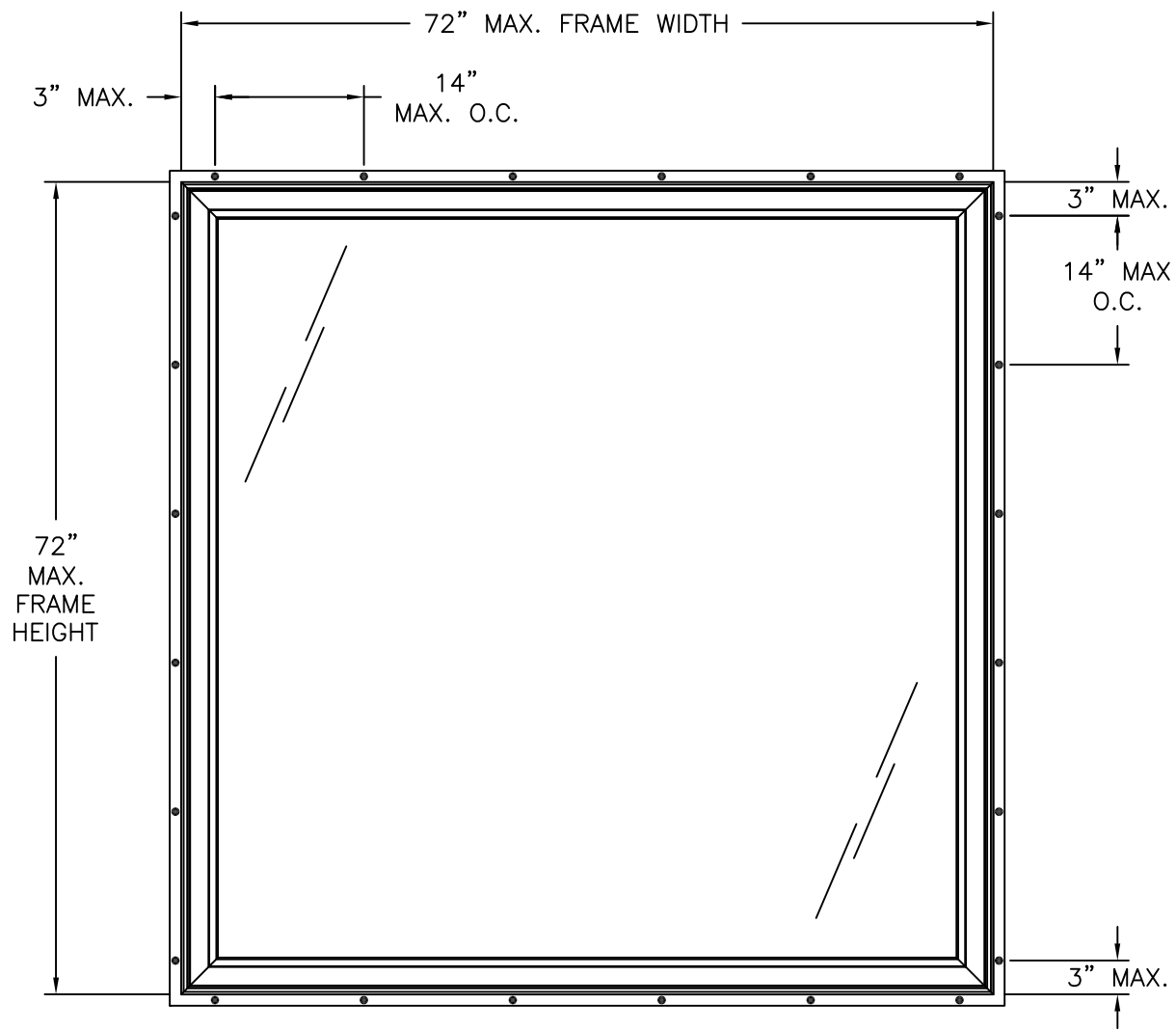
S-SERIES CASEMENT PICTURE EXTERIOR VIEW FIN INSTALLATION
