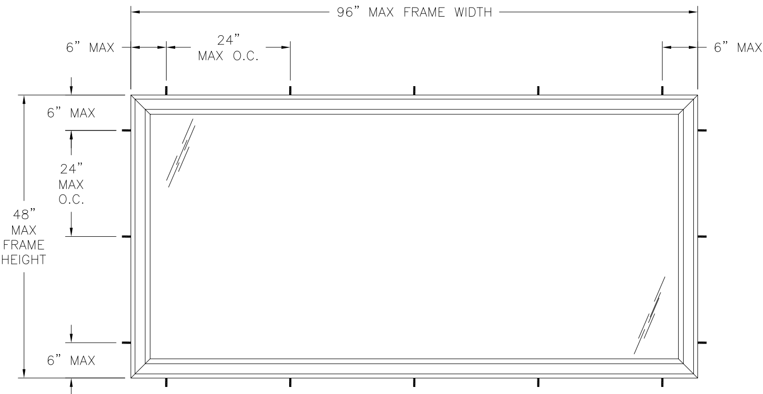
OCEANVIEW IMPACT SGD FIXED TRANSOM EXTERIOR VIEW FRAME INSTALLATION
