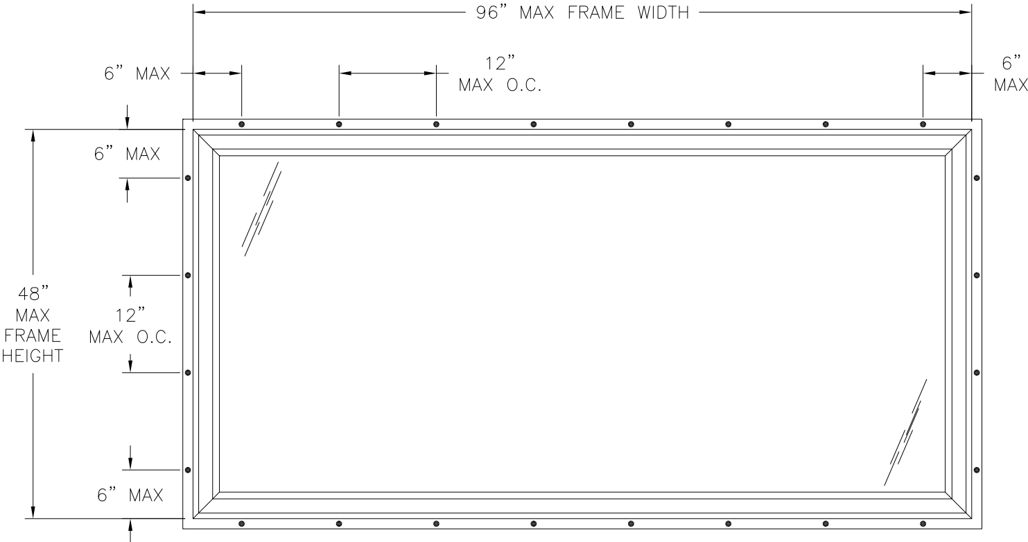
OCEANVIEW IMPACT SGD FIXED TRANSOM EXTERIOR VIEW FIN INSTALLATION
