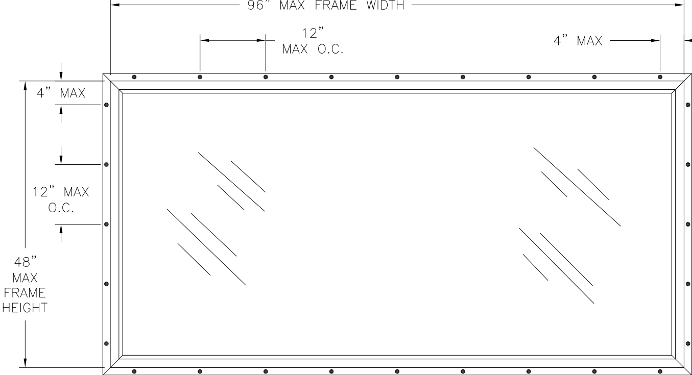
OCEANVIEW GEOMETRIC IMPACT PICTURE WINDOW EXTERIOR VIEW FIN INSTALLATION
