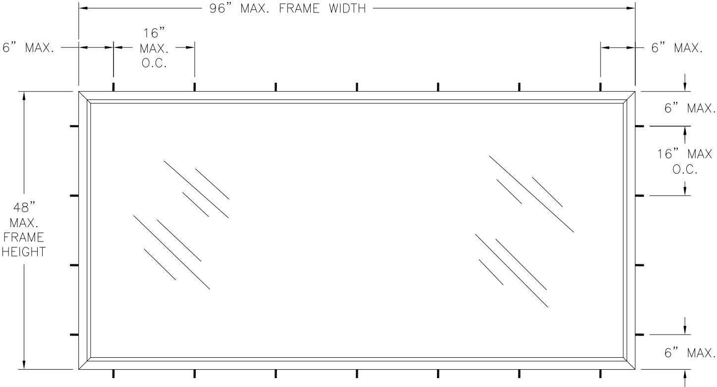
OCEANVIEW GEOMETRIC IMPACT PICTURE WINDOW EXTERIOR VIEW FRAME INSTALLATION
