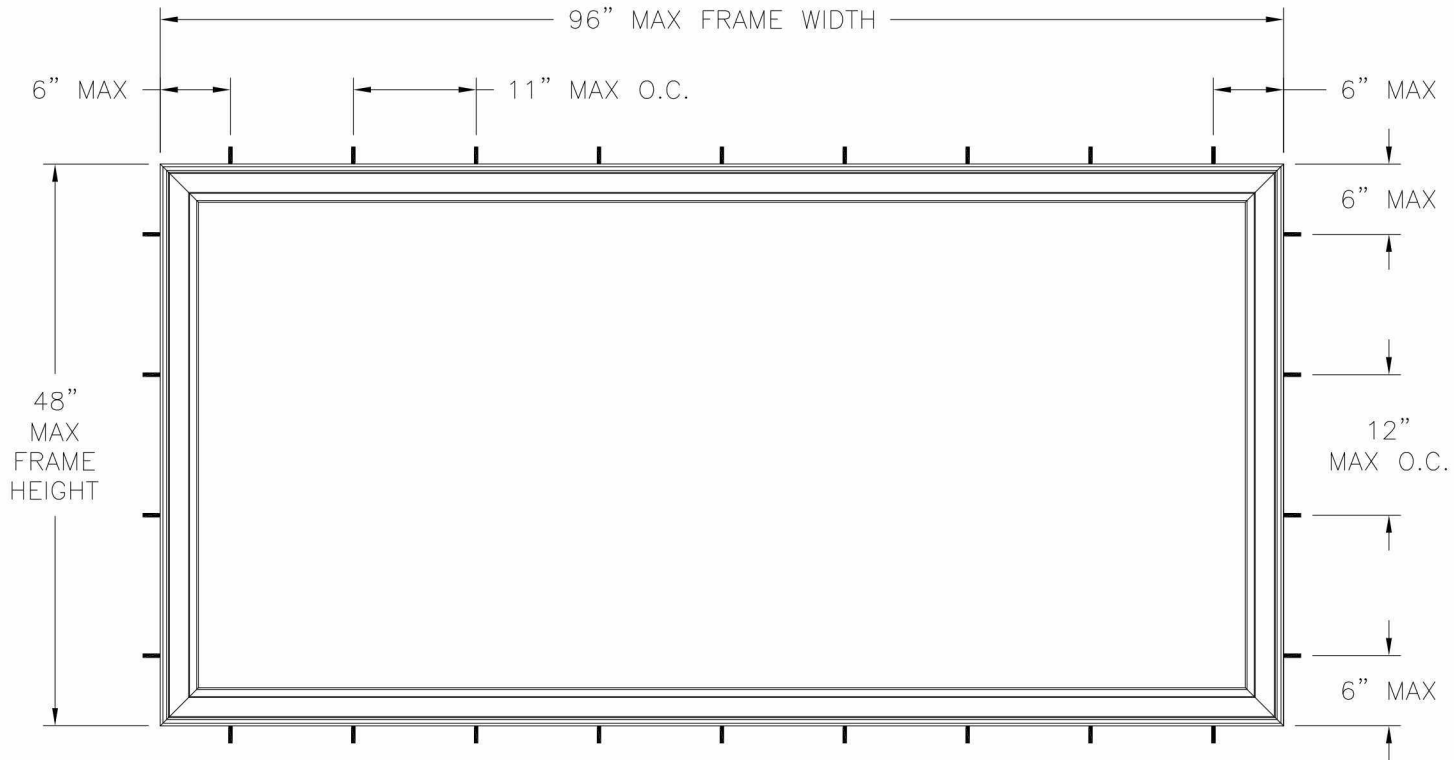
CAMBRIDGE FIXED EXTERIOR VIEW FRAME INSTALLATION
