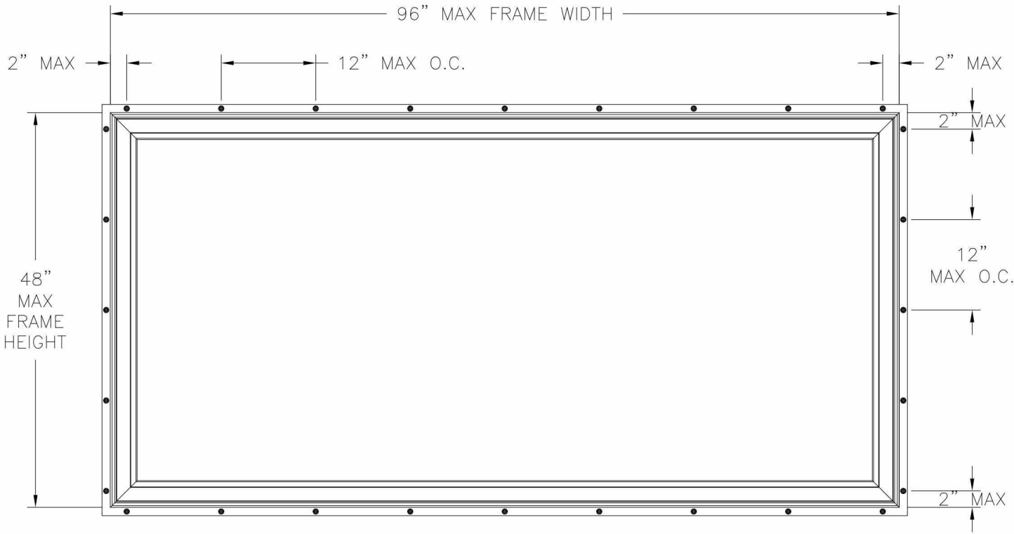
S-SERIES FIXED EXTERIOR VIEW FIN INSTALLATION
