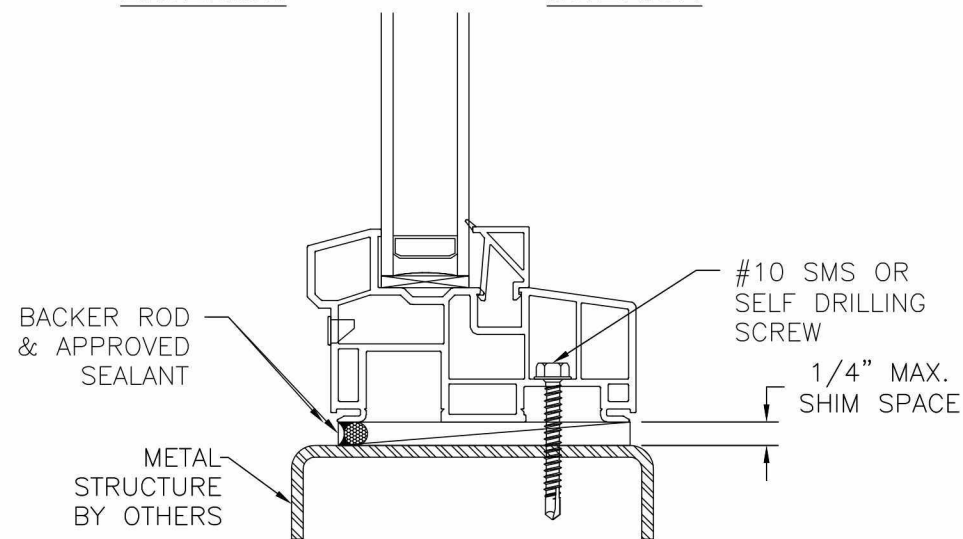
EXTERIOR INTERIOR
