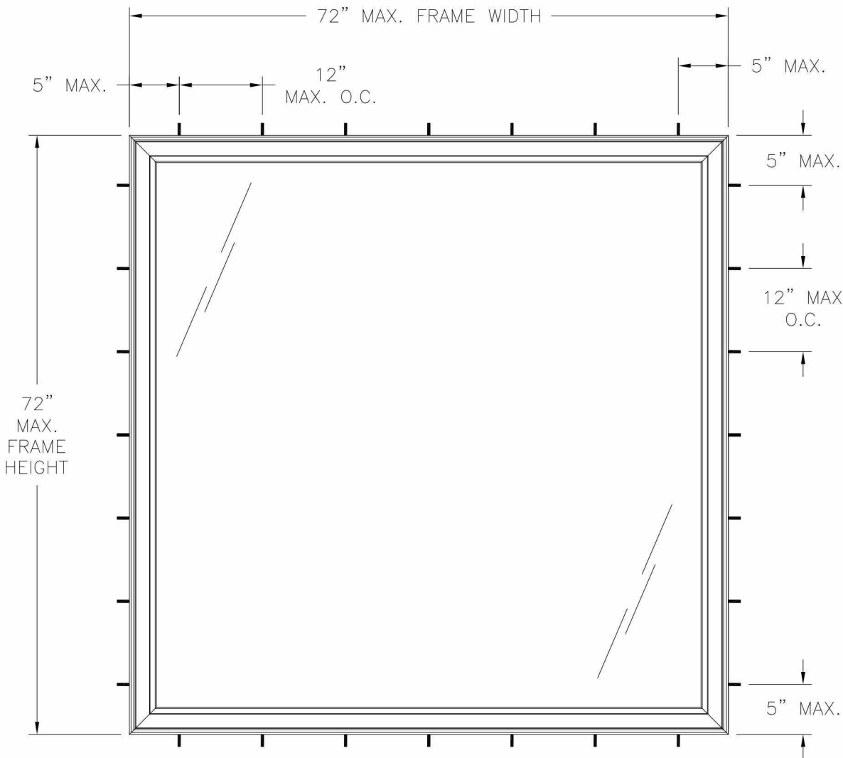
CAMBRIDGE CASEMENT PICTURE EXTERIOR VIEW FRAME INSTALLATION
