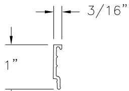
GLAZING BEAD V-663 RIGID PVC .050" THICK
