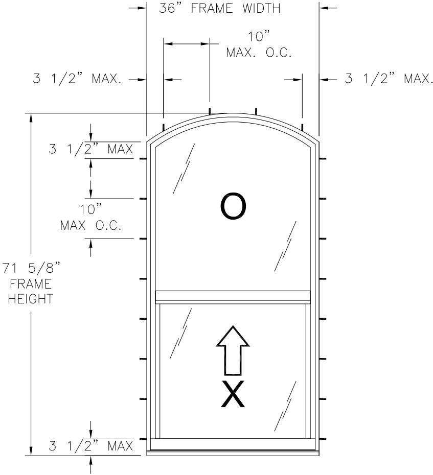
185 ALUMINUM SINGLE HUNG WINDOW DESIGNER EXTERIOR VIEW FLANGE & FINLESS INSTALLATION
