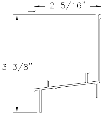
FLANGE FRAME SILL CM-18502 ALUMINUM 6063-T5 .055" THICK
