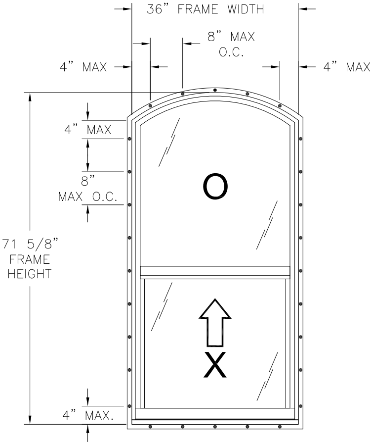
185 ALUMINUM SINGLE HUNG WINDOW DESIGNER EXTERIOR VIEW FIN INSTALLATION
