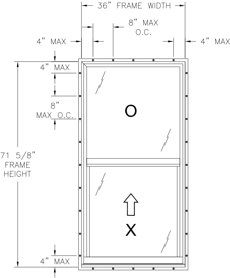
185 ALUMINUM SINGLE HUNG WINDOW EXTERIOR VIEW FIN INSTALLATION
