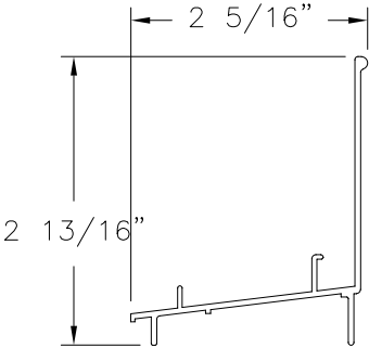
FINLESS FRAME SILL CM-18554 ALUMINUM 6063-T5 .055" THICK
