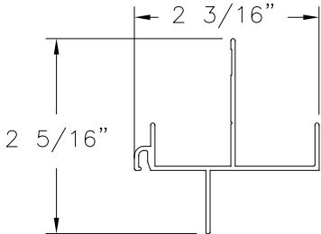
FIN FRAME HEAD CM-18508 ALUMINUM 6063-T5 .050" THICK
