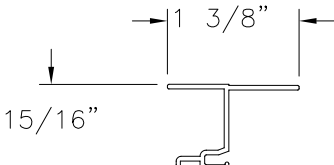
SASH STILE CM-18507 ALUMINUM 6063-T5 .050" THICK
