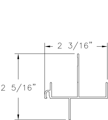
FIN FRAME HEAD CM-18508 ALUMINUM 6063-T5 .050" THICK
