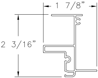
FLANGE FRAME JAMB CM-18503 ALUMINUM 6063-T5 .050" THICK
