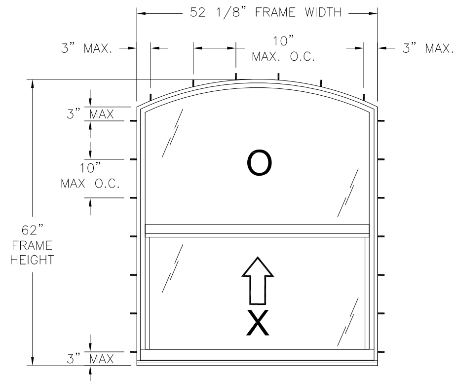
185 ALUMINUM SINGLE HUNG WINDOW DESIGNER EXTERIOR VIEW FLANGE & FINLESS INSTALLATION
