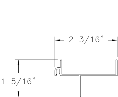
FINLESS FRAME HEAD CM-18553 ALUMINUM 6063-T5 .050" THICK
