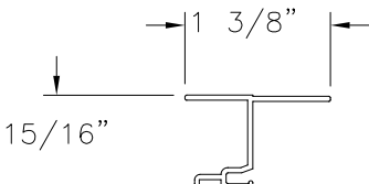
SASH STILE CM-18507 ALUMINUM 6063-T5 .050" THICK
