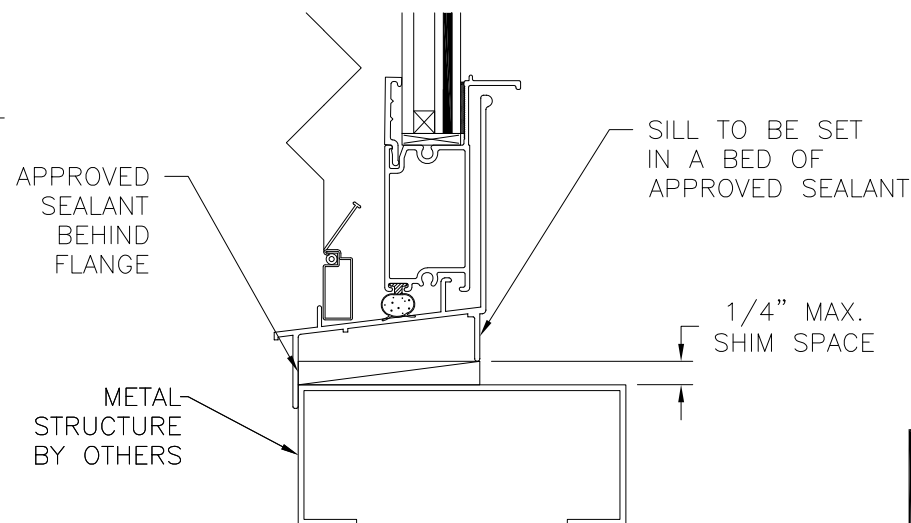
VERTICAL CROSS SECTION METAL STRUCTURE INSTALLATION
