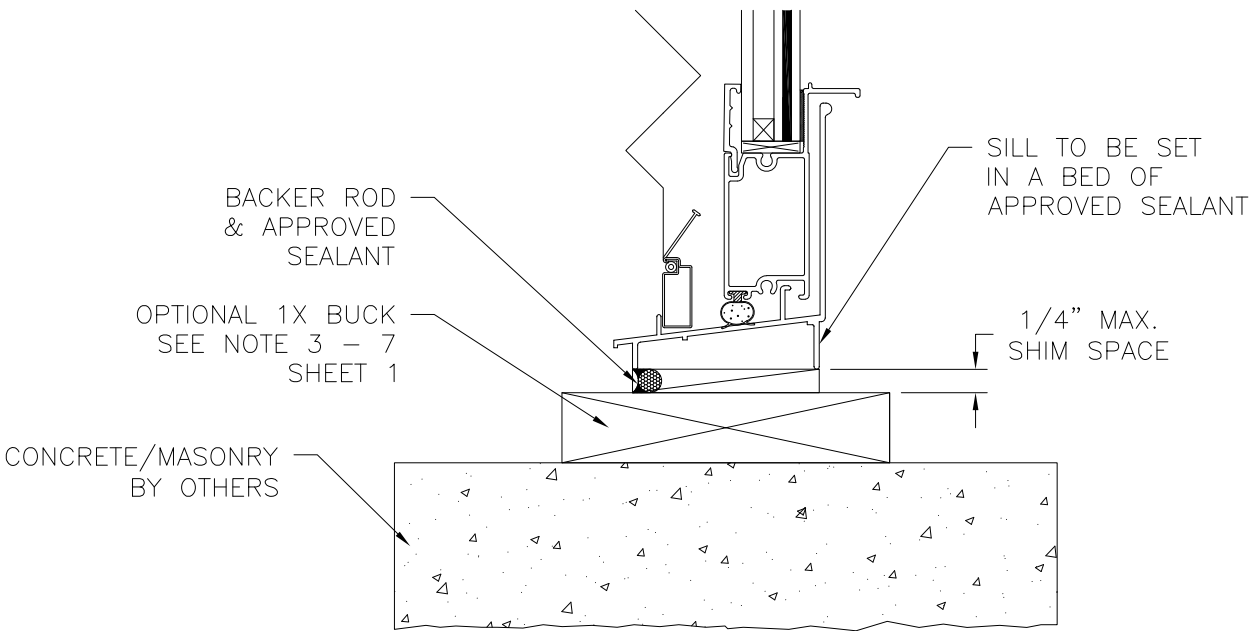
VERTICAL CROSS SECTION CONCRETE/MASONRY INSTALLATION
