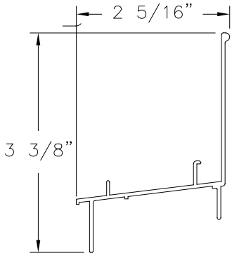
FLANGE FRAME SILL CM-18502 ALUMINUM 6063-T5 .055" THICK
