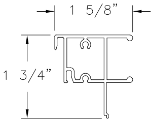
LOCK RAIL/STILE CM-18505 ALUMINUM 6063-T5 .062" THICK
