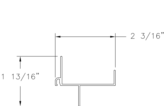
FLANGE FRAME HEAD CM-18501 ALUMINUM 6063-T5 .050" THICK
