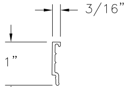
GLAZING BEAD V-663 RIGID PVC .070" THICK
