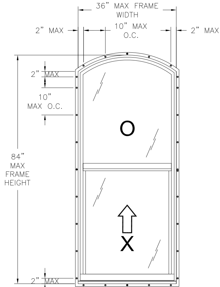
185 ALUMINUM SINGLE HUNG WINDOW
