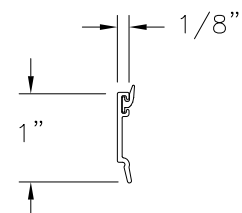
GLAZING BEAD CM-18535 RIGID PVC .050" THICK
