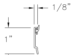
GLAZING BEAD CM-18535 RIGID PVC .050" THICK
