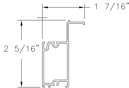
SASH BOTTOM RAIL CM-18555 ALUMINUM 6063-T5 .050" THICK
