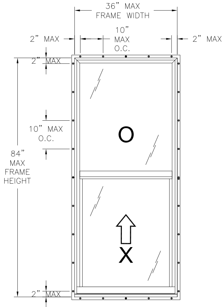
185 ALUMINUM SINGLE HUNG WINDOW
