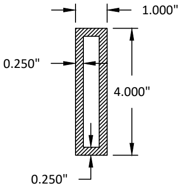
1" X 4" MULLION SEE SHEET 10 FOR QUALIFIED CLIPS
