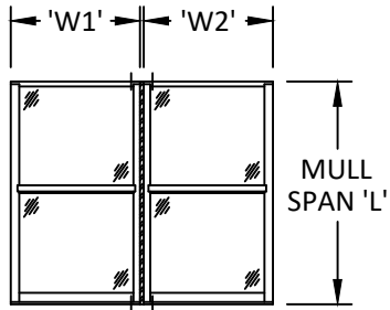
VERTICAL SPAN
