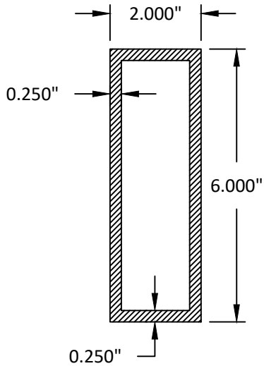
2" X 6" MULLION SEE SHEET 12 FOR QUALIFIED CLIPS
