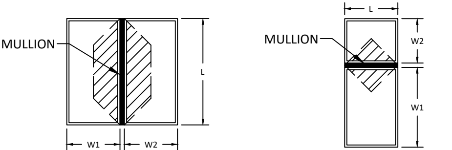
ONE-WAY MULLION DIAGRAMS
