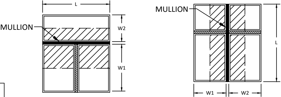
TWO-WAY MULLION DIAGRAMS
