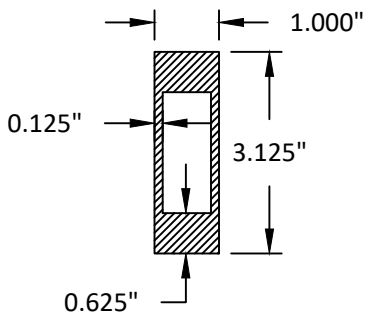
1" X 3-1/8" (HEAVY) MULLION SEE SHEET 9 FOR QUALIFIED CLIPS
