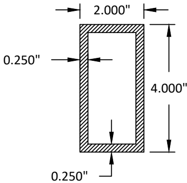
2" X 4" MULLION SEE SHEET 11 FOR QUALIFIED CLIPS
