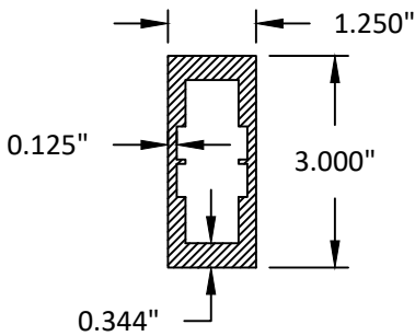
1-1/4" X 3" MULLION SEE SHEET 8 FOR QUALIFIED CLIPS
