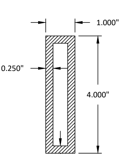
1" X 4" MULLION
