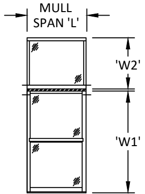
HORIZONTAL SPAN
