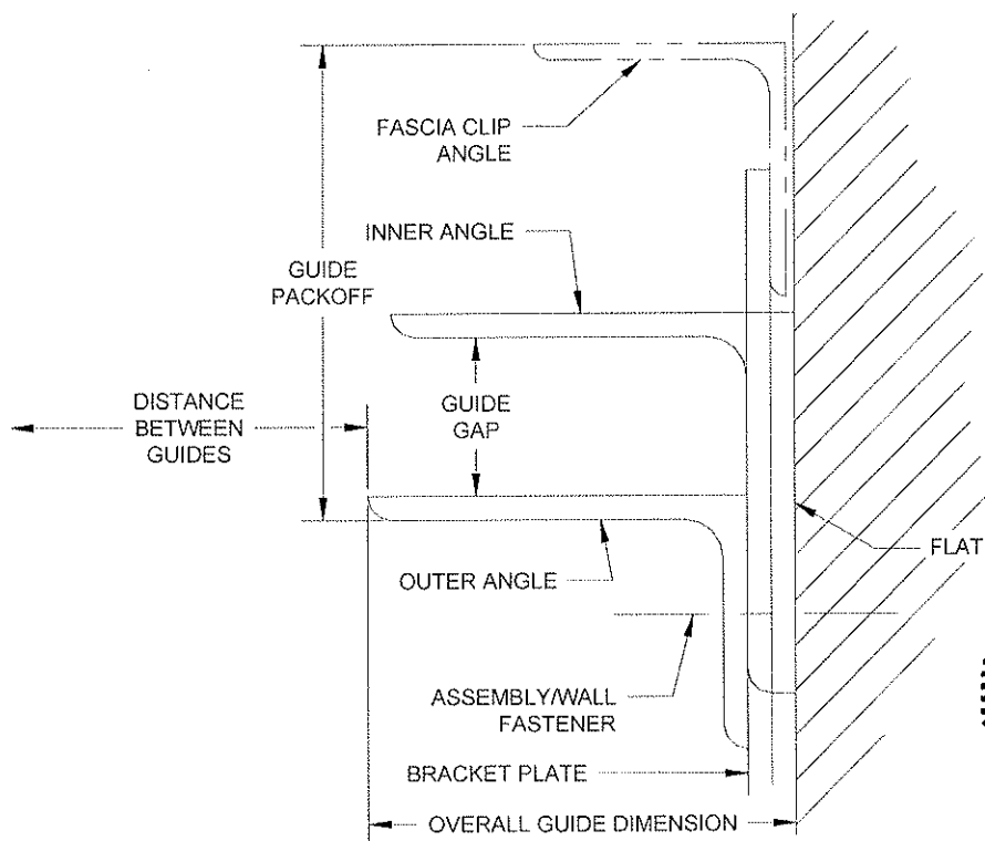
Figure 5.9 – Between Jamb Two-Angle Guide with Flat
