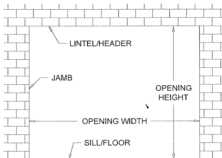
Figure 4.1 - Opening Dimensions and Designations
