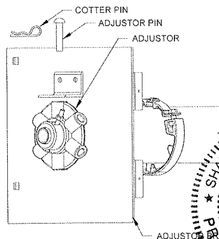
Figure 8.5 – Pinning the Adjusting Wheel
