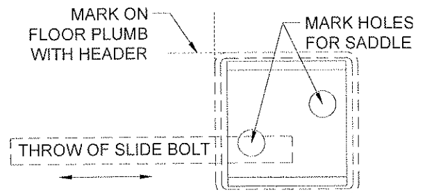
Figure 5.13 – Tube Saddle Hole location
