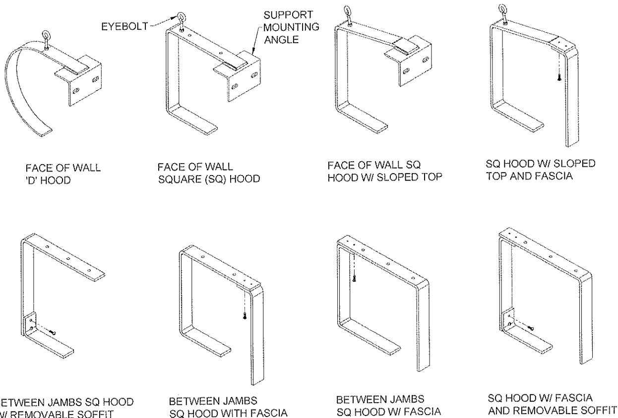
Figure 10.1 - Hood Supports
