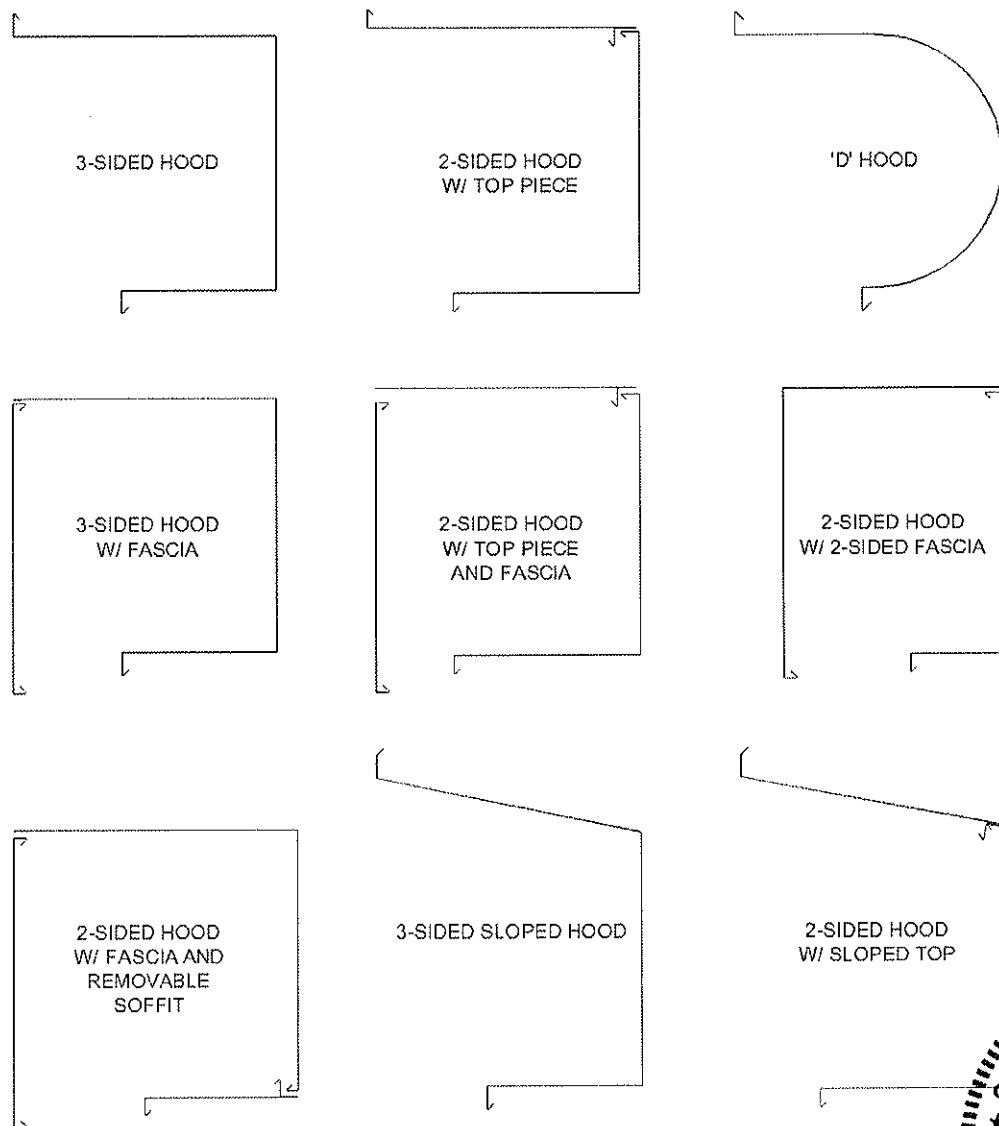
Figure 11.1 - Hood Configurations
