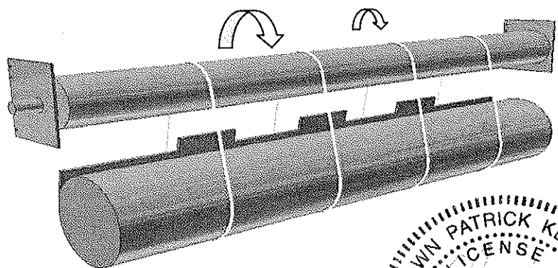
Figure 8.2 - Slinging the Curtain
