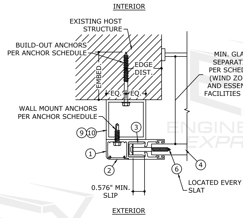
2 5 END RETENTION TYP. BUILD-OUT MOUNT N.T.S. HORIZ SECTION
