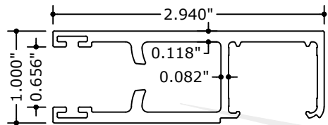
SNAP RAIL
