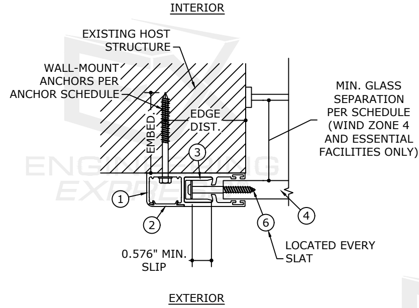
1 5 END RETENTION TYPICAL WALL MOUNT N.T.S. HORIZ SECTION
