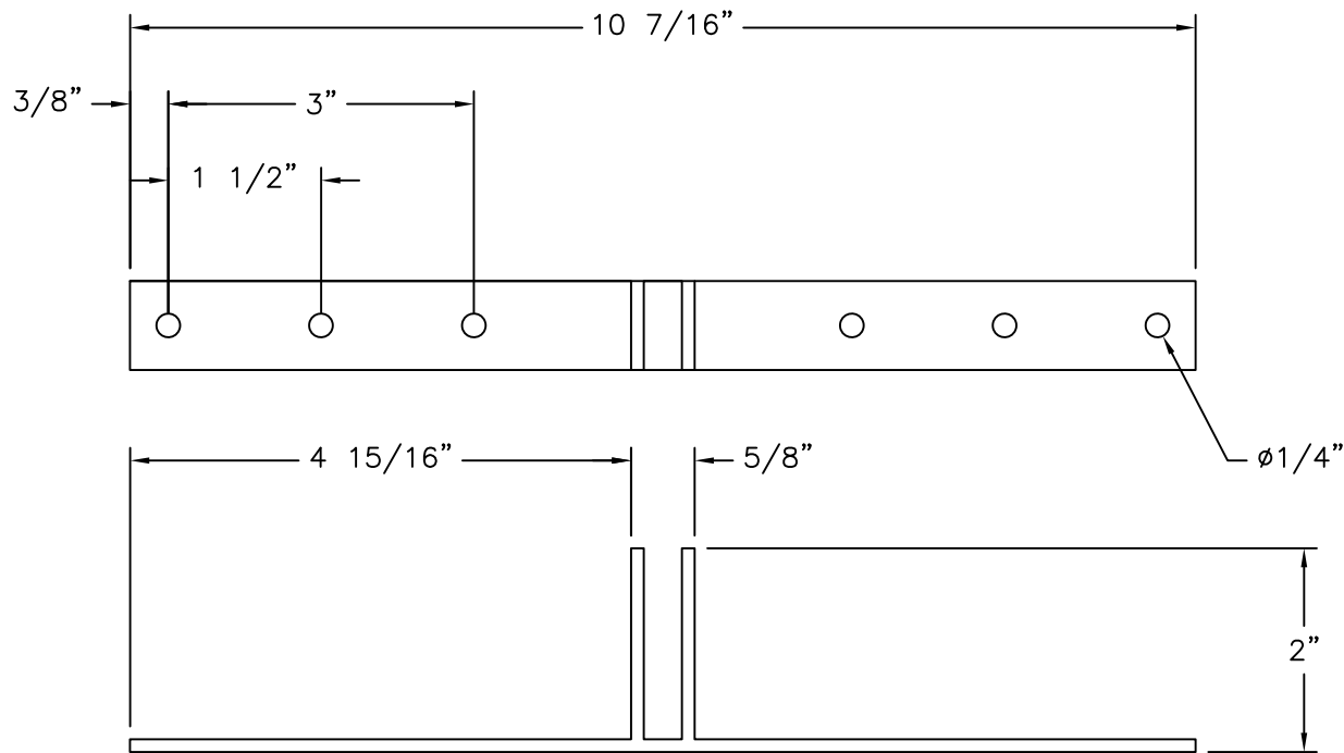
CLIP ALUMINUM 6063-T6 .125" THICK
