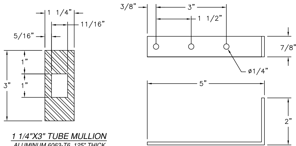
ANGLE ALUMINUM 6063-T6 .125" THICK
