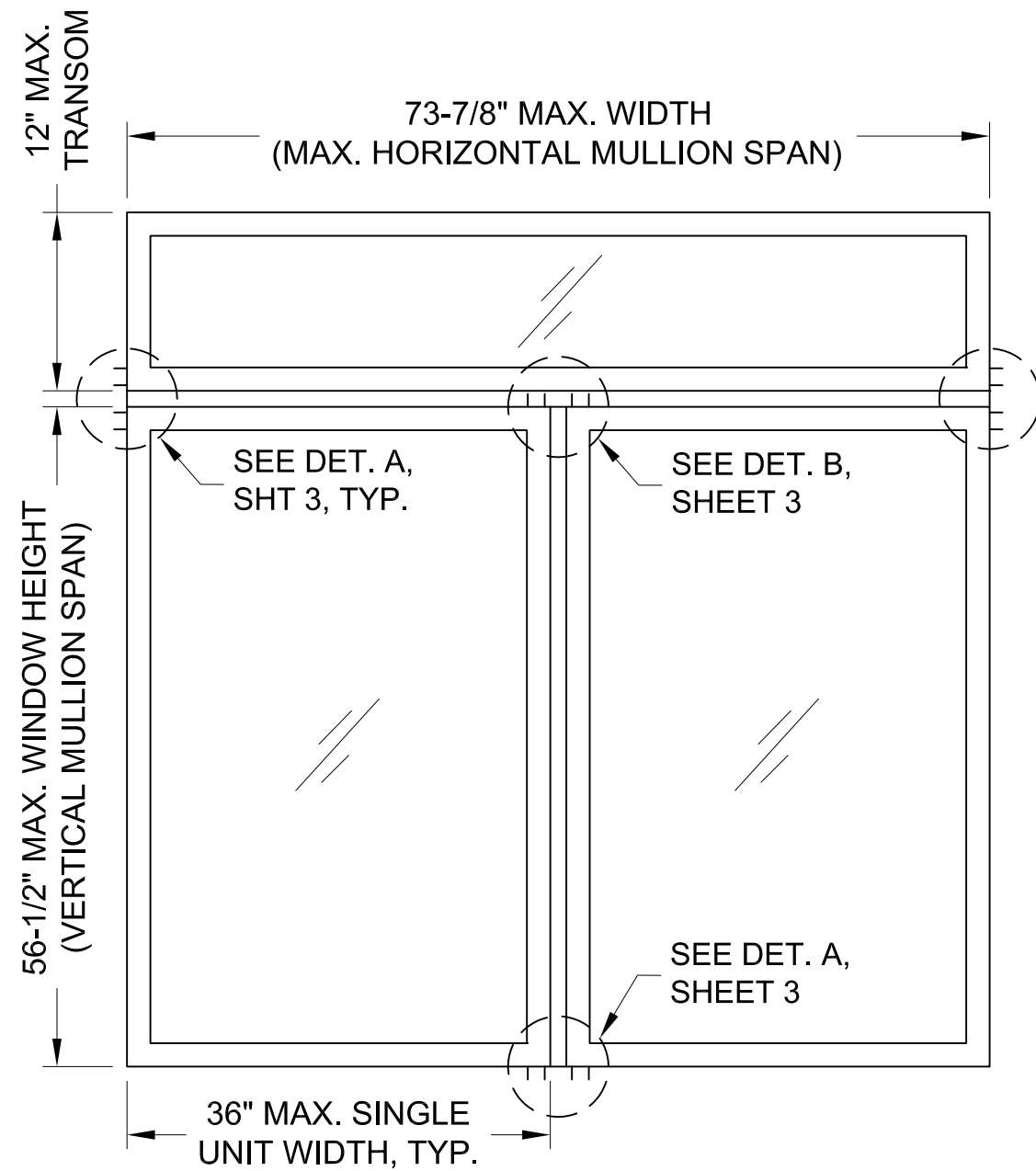
3" IMPACT VERTICAL / HORIZONTAL "T" MULLION
