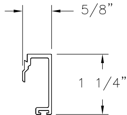
GLAZING BEAD ALUMINUM 6063-T5 .062" THICK
