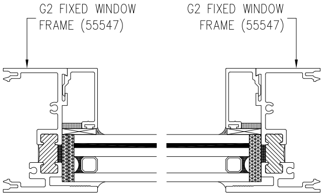
HORIZONTAL CROSS SECTION
