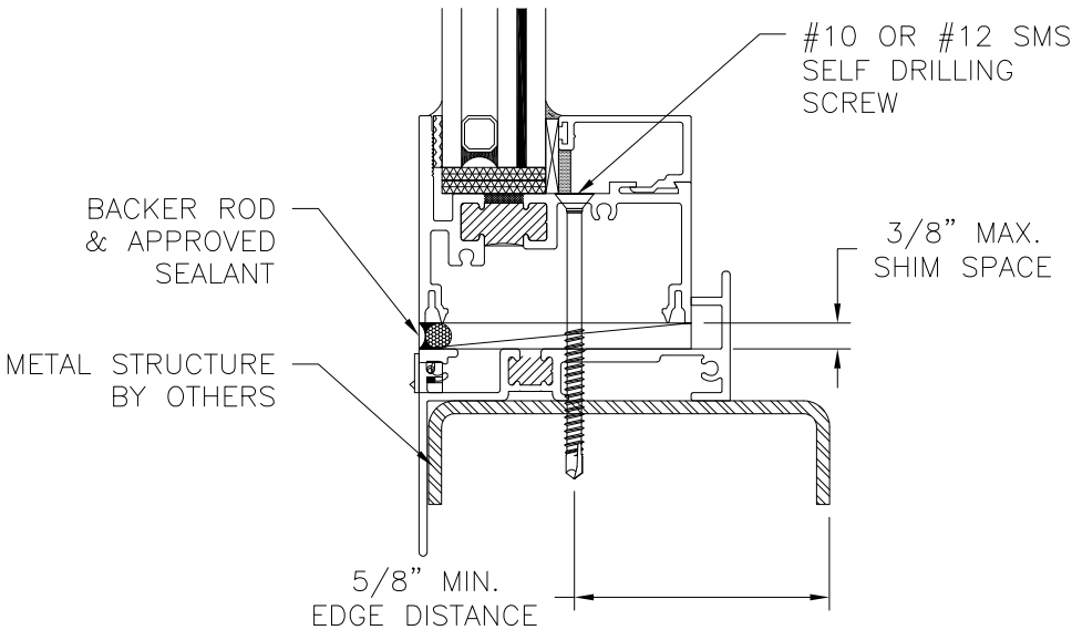
VERTICAL CROSS SECTION METAL STRUCTURE INSTALLATION WITH LOW PROFILE WINDOW PAN S67862
