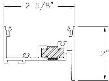
FRAME ALUMINUM 6063-T5 .100" THICK
