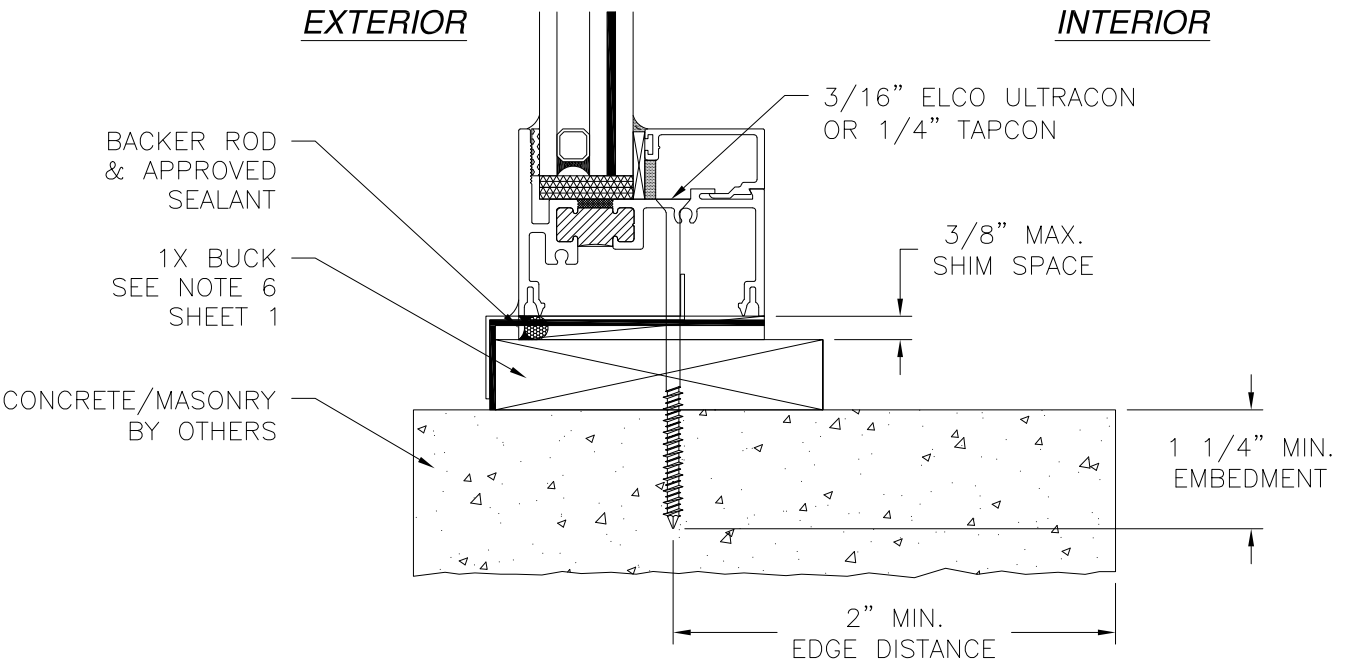
VERTICAL CROSS SECTION CONCRETE/MASONRY WITH 1X BUCK INSTALLATION FOR CONCRETE/MASONRY WITHOUT 1X BUCK REFER TO JAMB INSTALLATION DETAIL FOR ADDITIONAL SILL DETAIL, SEE SHEET 8
