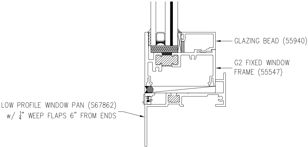
ADDITIONAL SILL DETAIL
