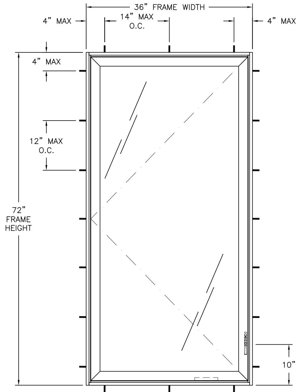
SERIES SI7000 G2 INTERNATIONAL CASEMENT WINDOW EXTERIOR VIEW
