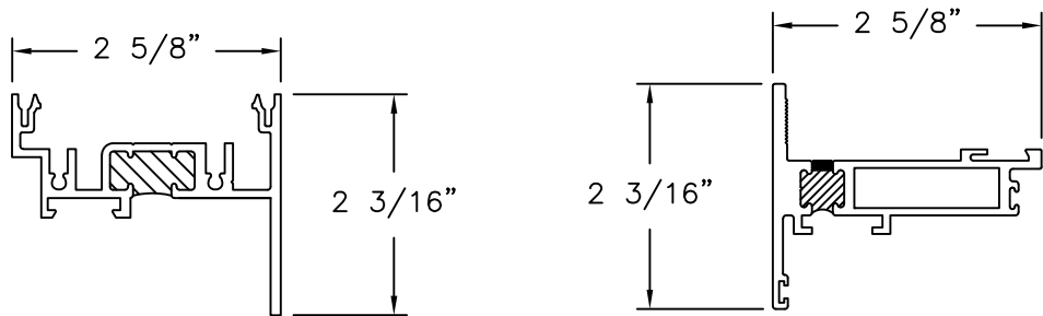
FRAME ALUMINUM 6063-T5 .100" THICK
