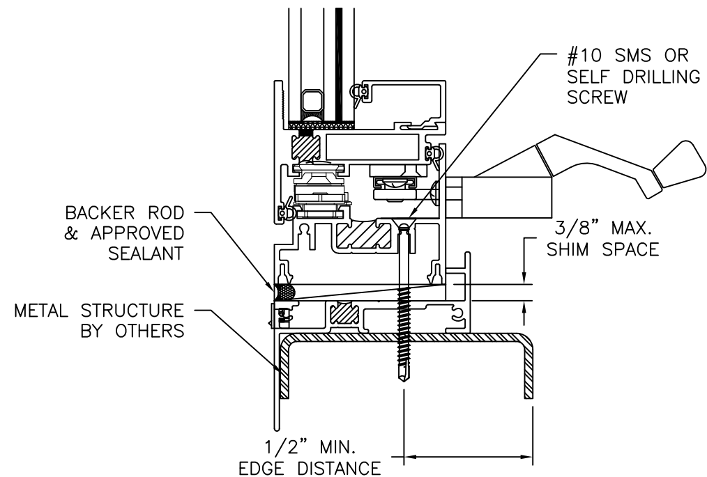
VERTICAL CROSS SECTION METAL STRUCTURE INSTALLATION WITH LOW PROFILE WINDOW PAN S67862
