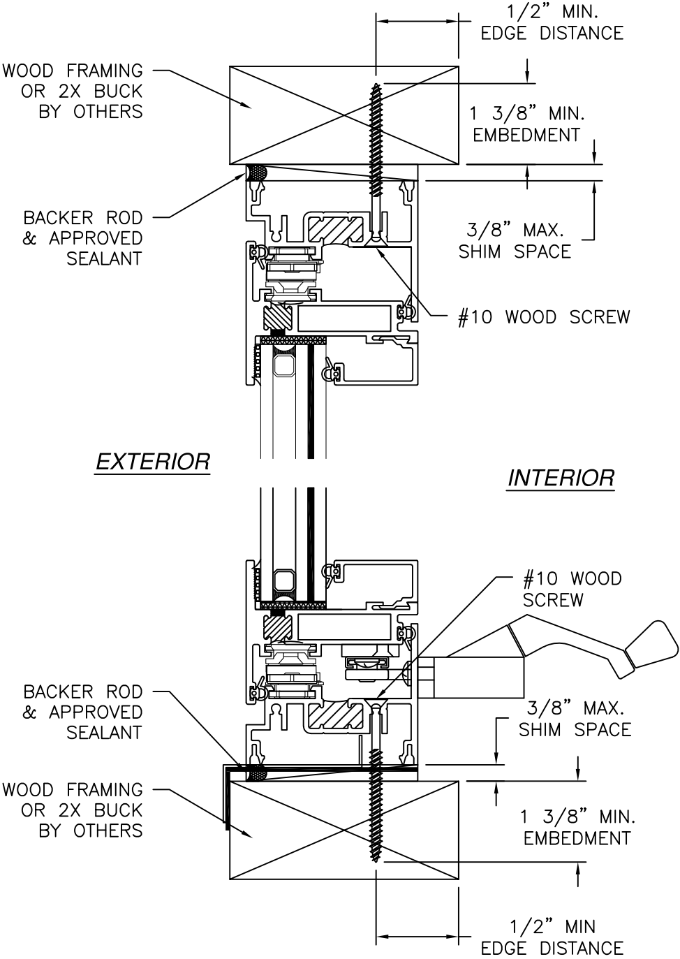
VERTICAL CROSS SECTION WOOD FRAMING OR 2X BUCK INSTALLATION FOR ADDITIONAL SILL DETAIL, SEE SHEET 8
