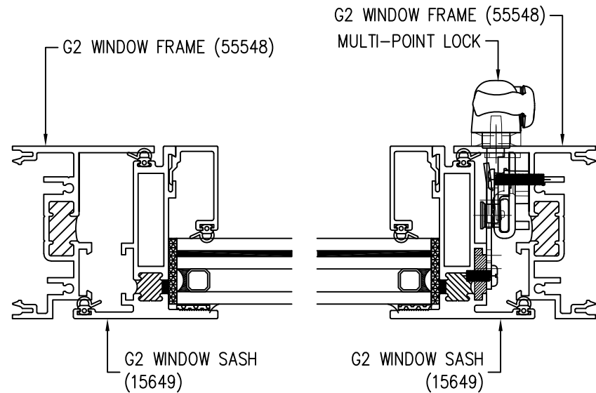
HORIZONTAL CROSS SECTION
