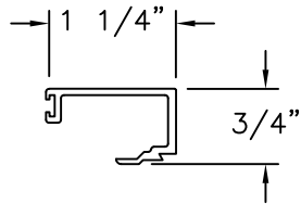
GLASS STOP ALUMINUM 6063-T5 .062" THICK
