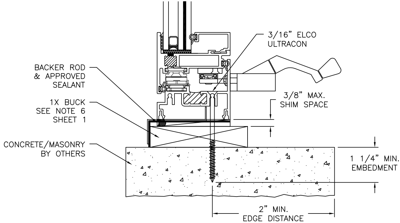
VERTICAL CROSS SECTION CONCRETE/MASONRY WITH 1X BUCK INSTALLATION FOR CONCRETE/MASONRY WITHOUT 1X BUCK REFER TO JAMB INSTALLATION DETAIL FOR ADDITIONAL SILL DETAIL, SEE SHEET 8
