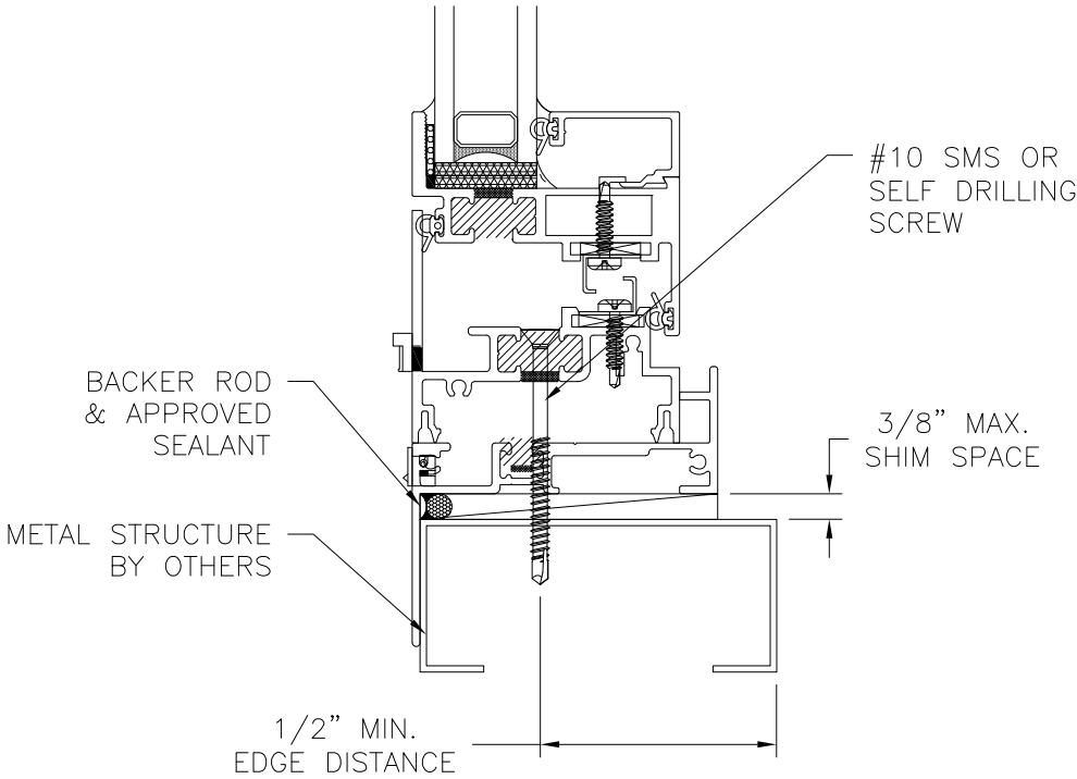
VERTICAL CROSS SECTION METAL STRUCTURE INSTALLATION WITH LOW PROFILE WINDOW PAN S67862
