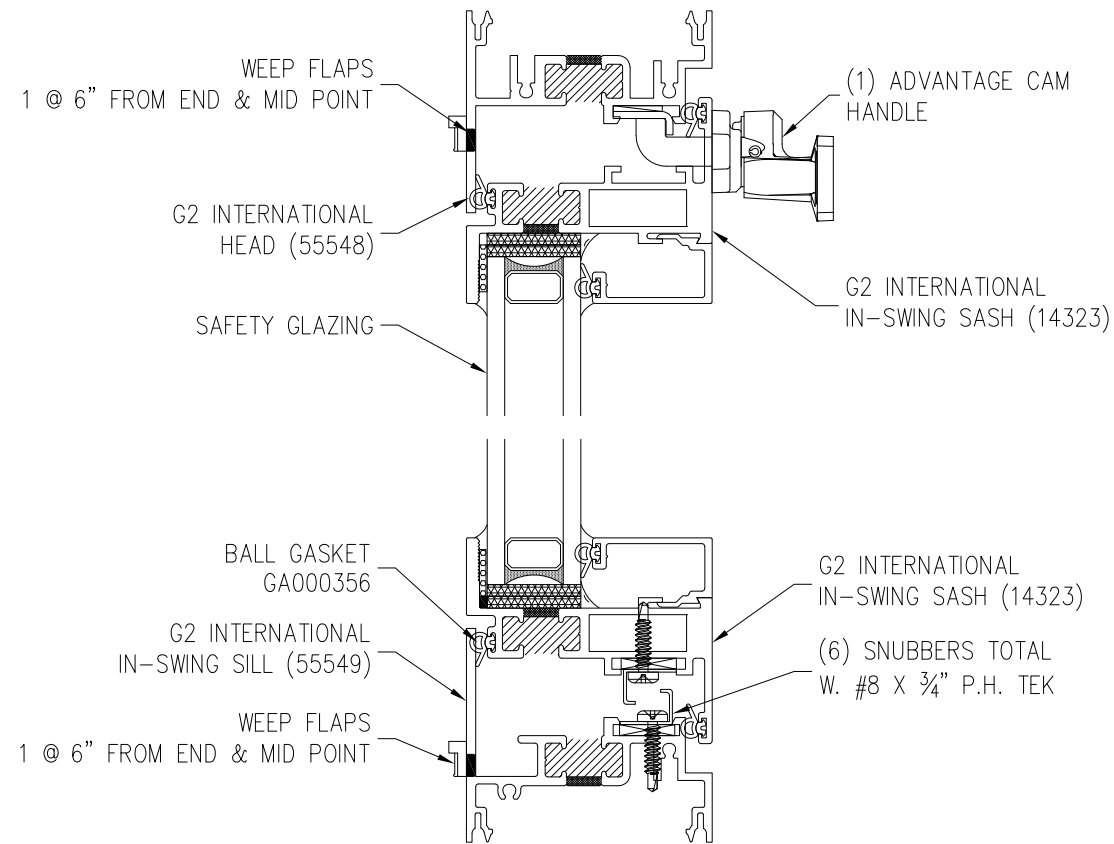
VERTICAL CROSS SECTION
