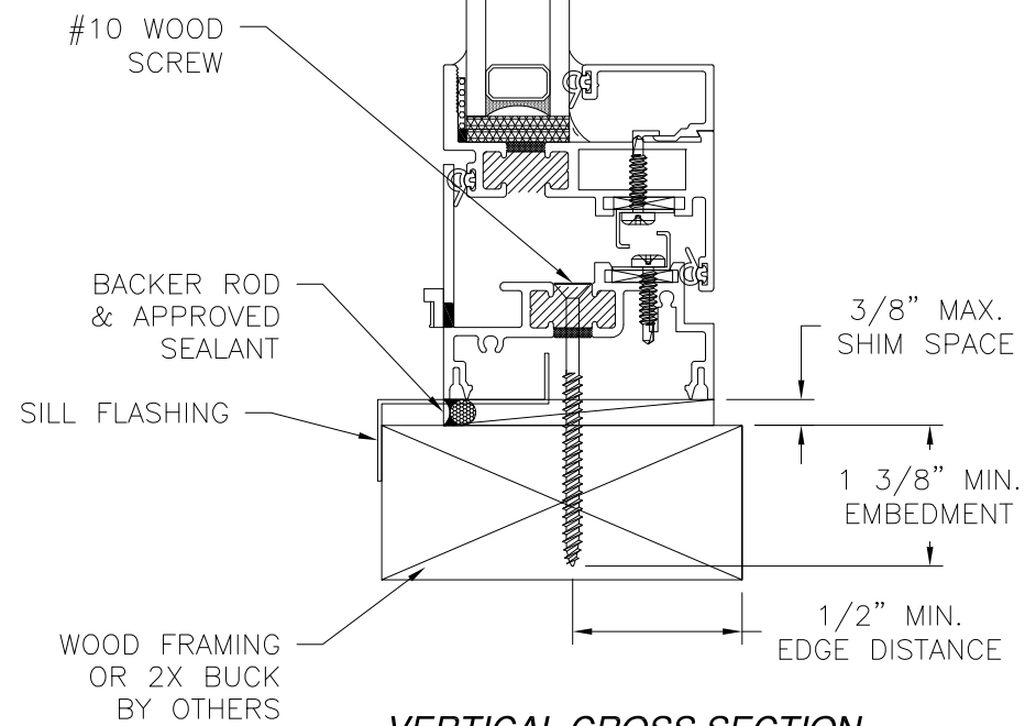
VERTICAL CROSS SECTION WOOD FRAMING OR 2X BUCK INSTALLATION FOR ADDITIONAL SILL DETAIL, SEE SHEET 7
