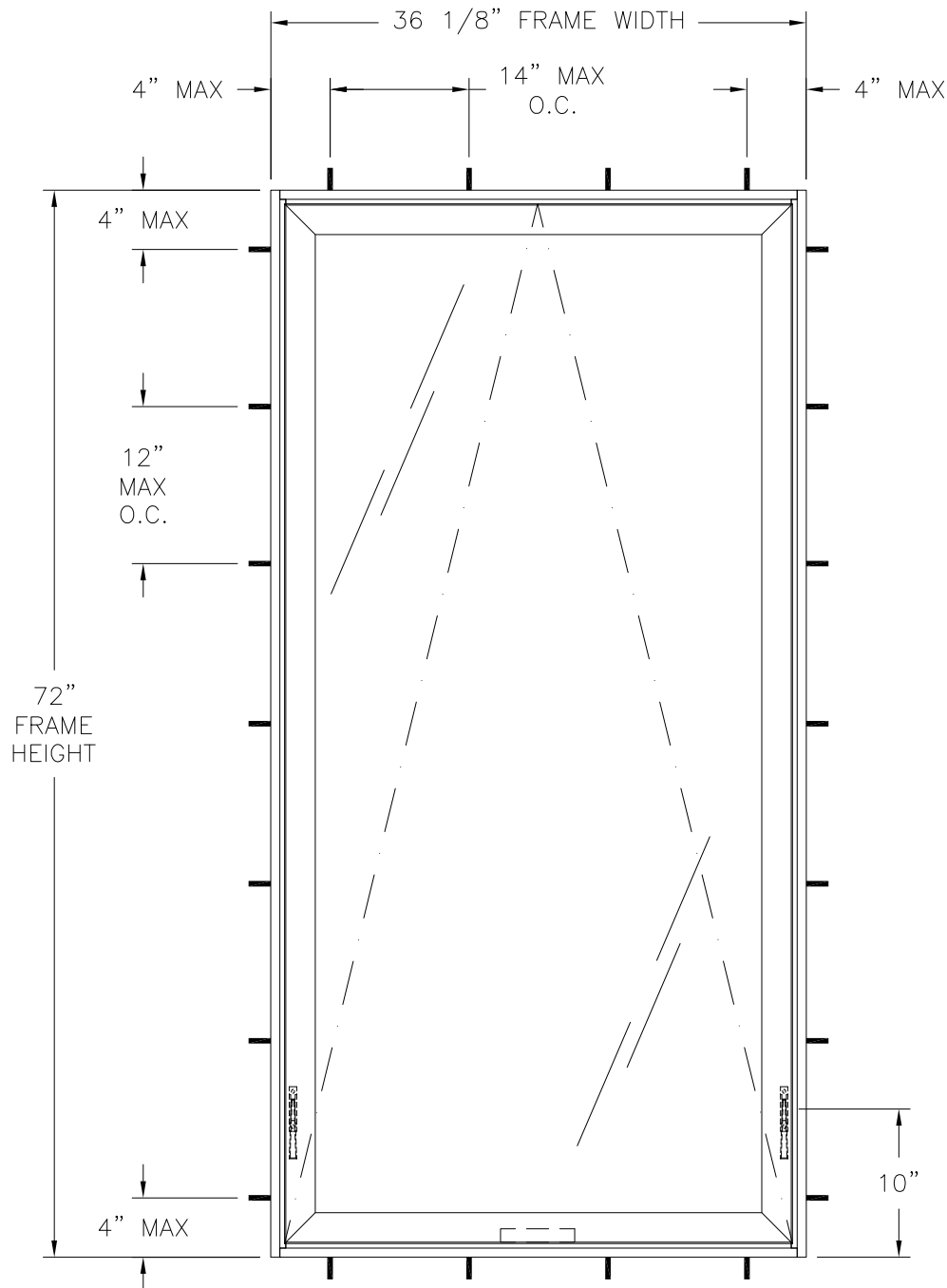
SERIES SI7000 G2 INTERNATIONAL AWNING WINDOW EXTERIOR VIEW
