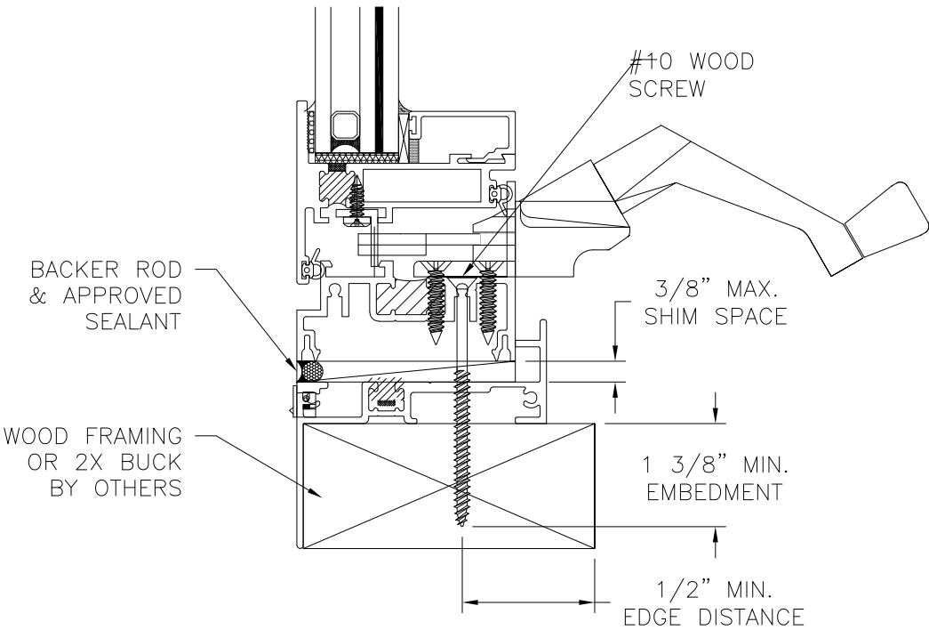
VERTICAL CROSS SECTION WOOD FRAMING OR 2X BUCK INSTALLATION WITH LOW PROFILE WINDOW PAN S67862
