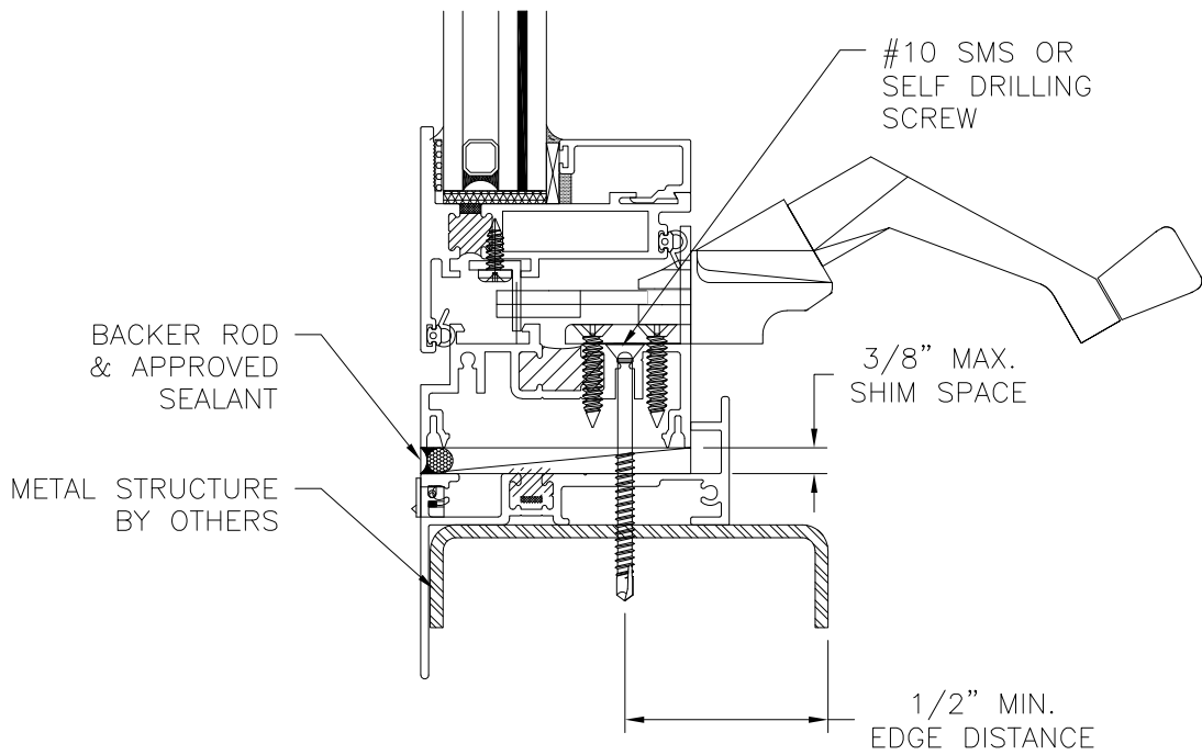
VERTICAL CROSS SECTION METAL STRUCTURE INSTALLATION WITH LOW PROFILE WINDOW PAN S67862
