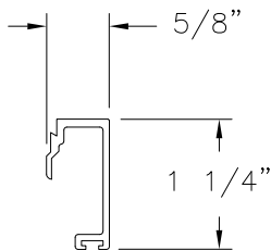
GLAZING BEAD ALUMINUM 6063-T5 .062" THICK
