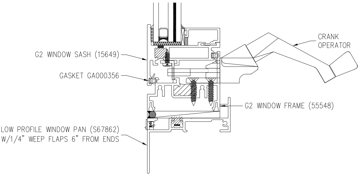
ADDITIONAL SILL DETAIL
