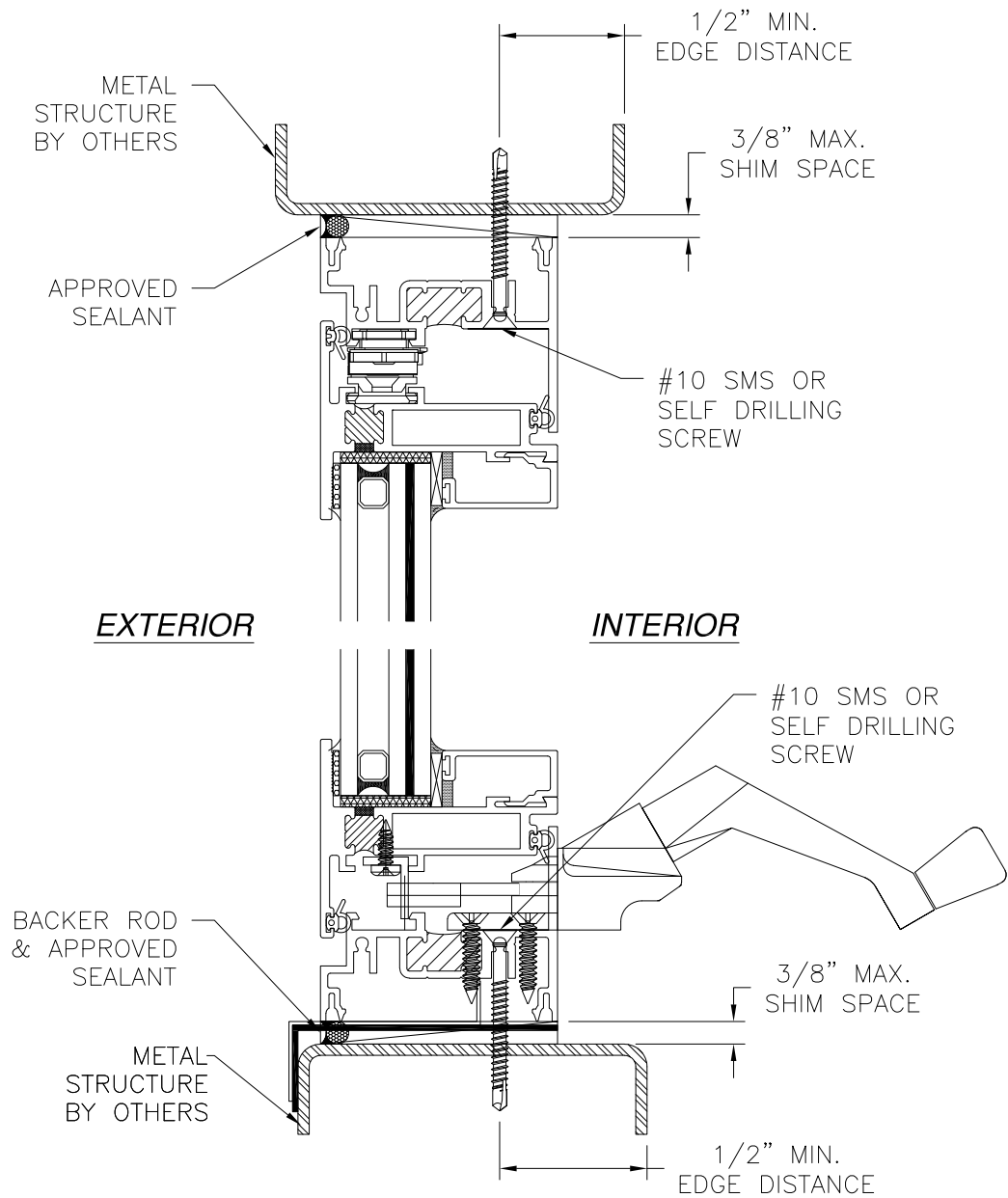
VERTICAL CROSS SECTION METAL STRUCTURE INSTALLATION FOR ADDITIONAL SILL DETAIL, SEE SHEET 8
