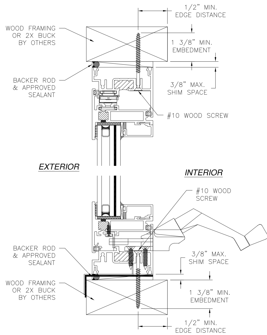
VERTICAL CROSS SECTION WOOD FRAMING OR 2X BUCK INSTALLATION FOR ADDITIONAL SILL DETAIL, SEE SHEET 8
