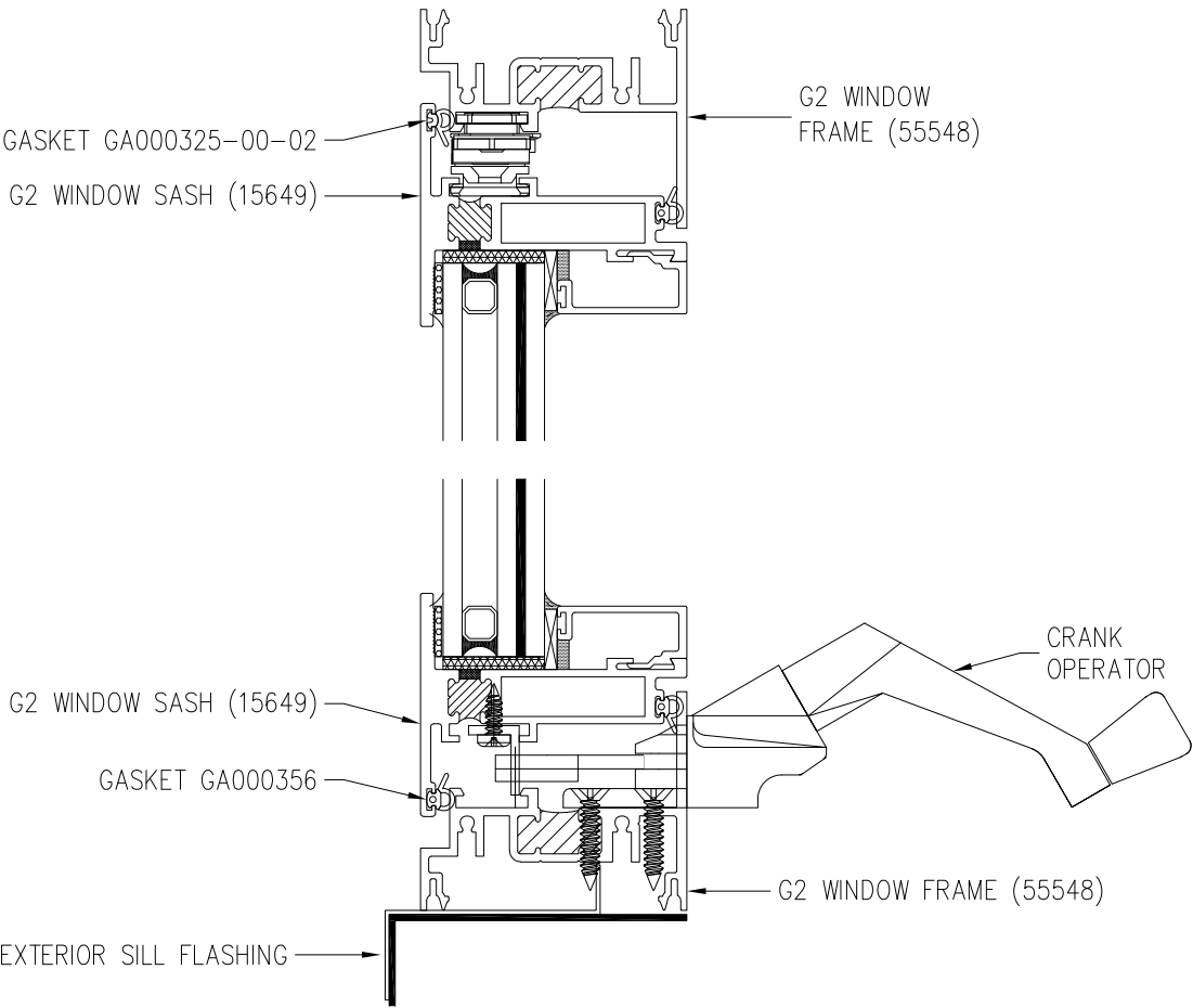
VERTICAL CROSS SECTION
