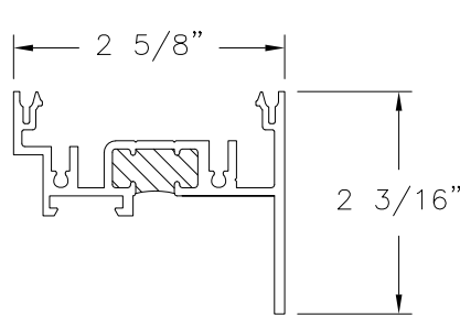
FRAME ALUMINUM 6063-T5 .100" THICK
