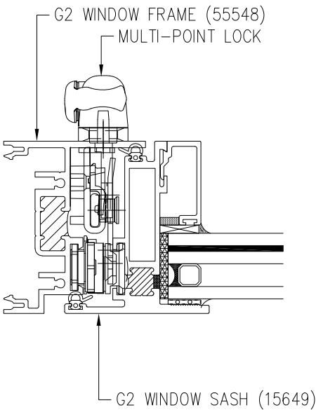
HORIZONTAL CROSS SECTION
