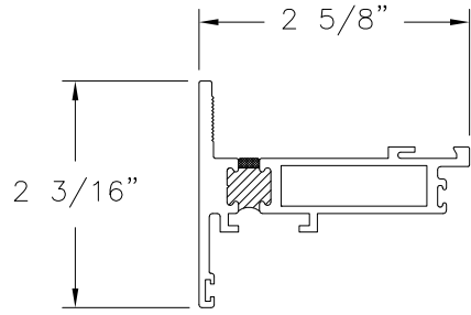
SASH ALUMINUM 6063-T5 .100" THICK
