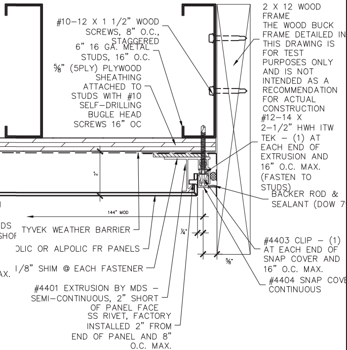
6 panel termination detail 6" = 1'-0" ref:
