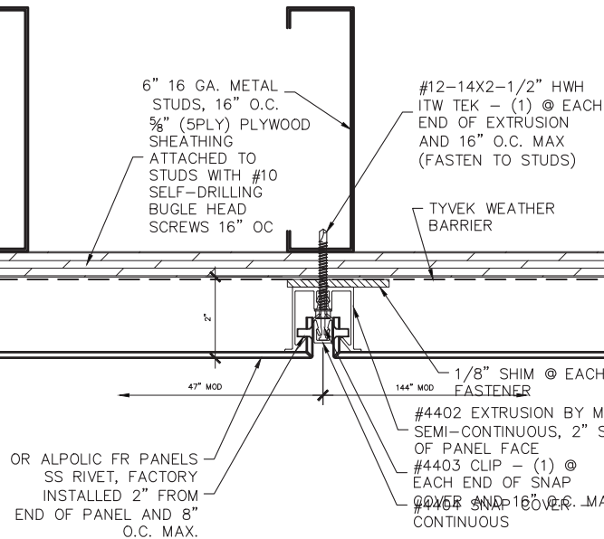
5 typ vertical panel joint detail 6" = 1'-0" ref:
