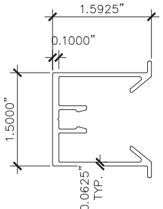
4-4402-00 FIELD EXTRUSION (MILL FINISHED ALUMINUM)
