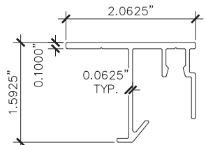
4-4401-00 PERIMETER EXTRUSION (MILL FINISH ALUMINUM)
