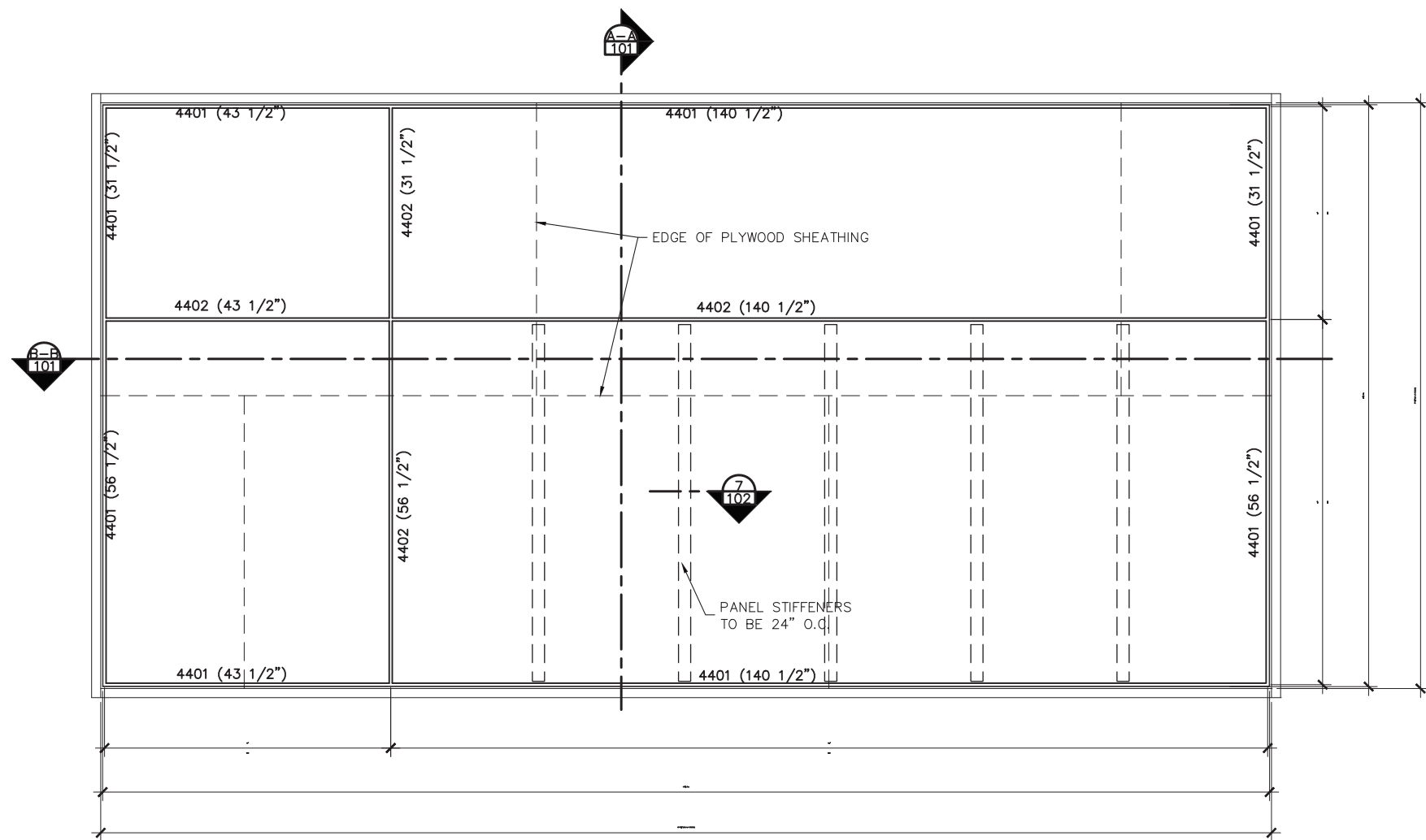
1 elevation 101 ref: 1" = 1'-0"
