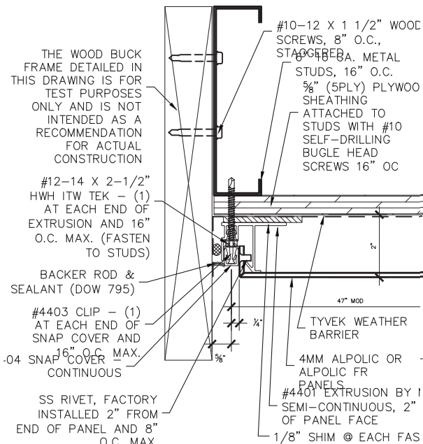
4 panel termination detail 6" = 1'-0" ref:
