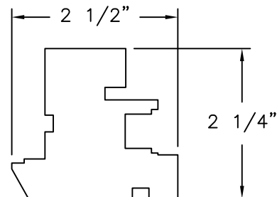
⑬ MEETING STILE MAHOGANY WOOD
