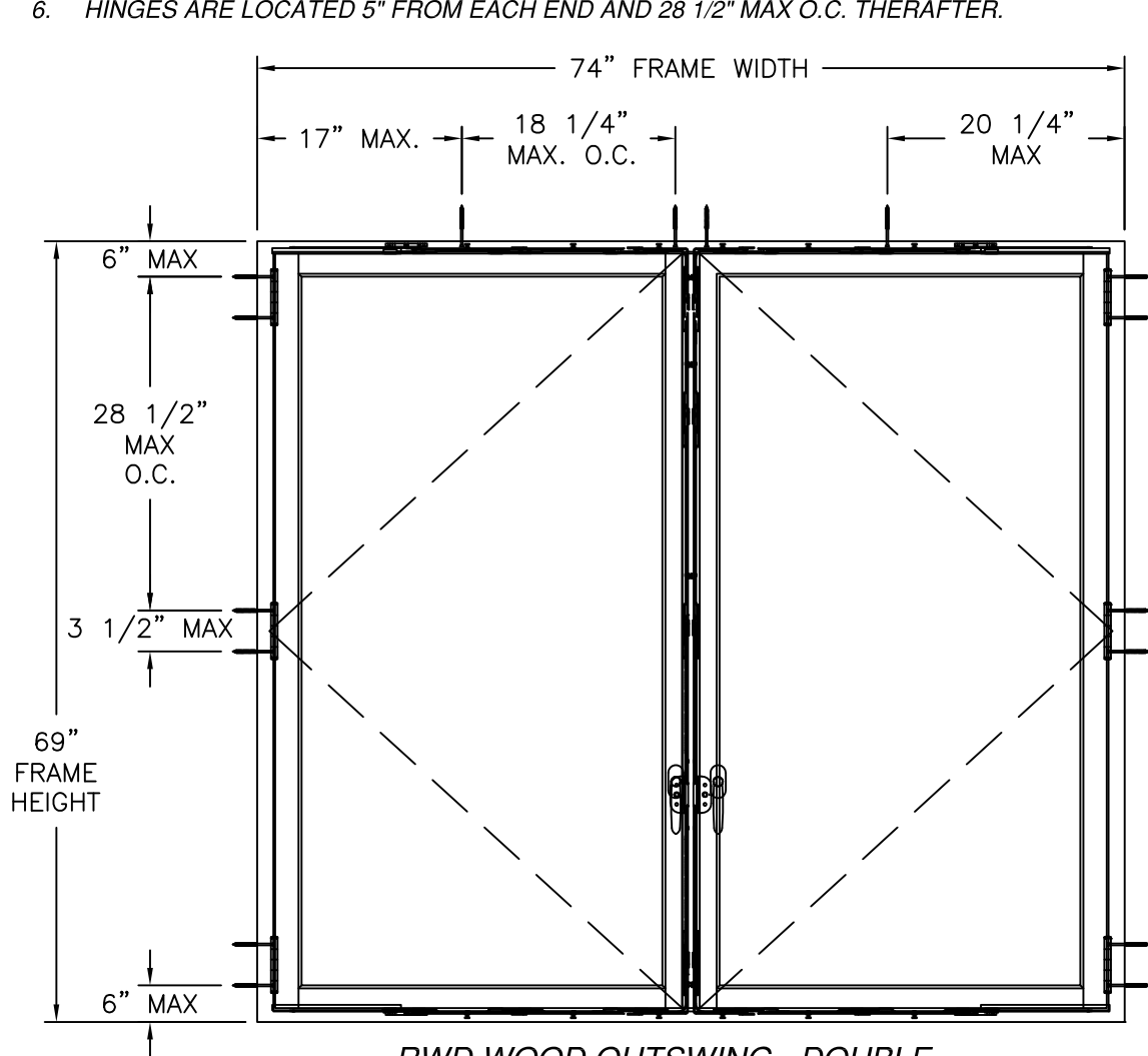
RWD WOOD OUTSWING - DOUBLE EXTERIOR VIEW (ANCHORS THROUGH HARDWARE & HINGES)
