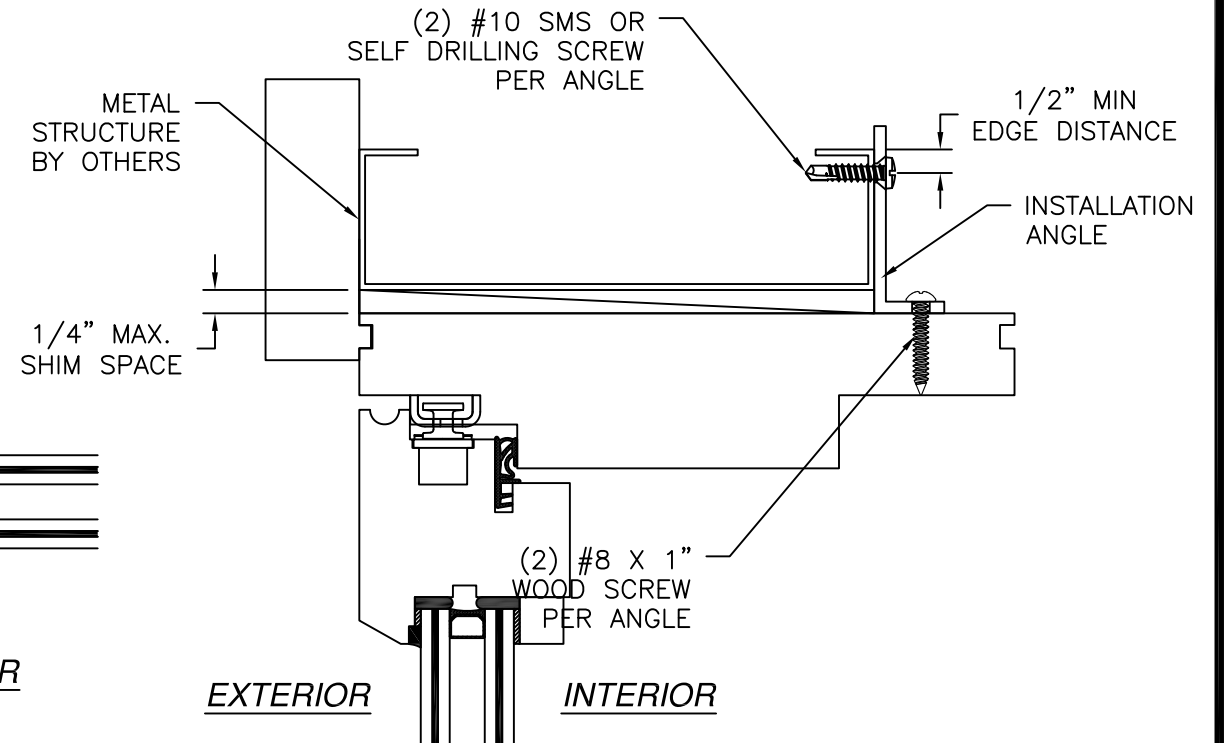
VERTICAL CROSS SECTION METAL STRUCTURE INSTALLATION
