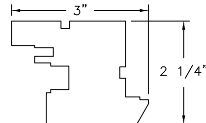
⑮ STILE (ASTRAGAL) MAHOGANY WOOD
