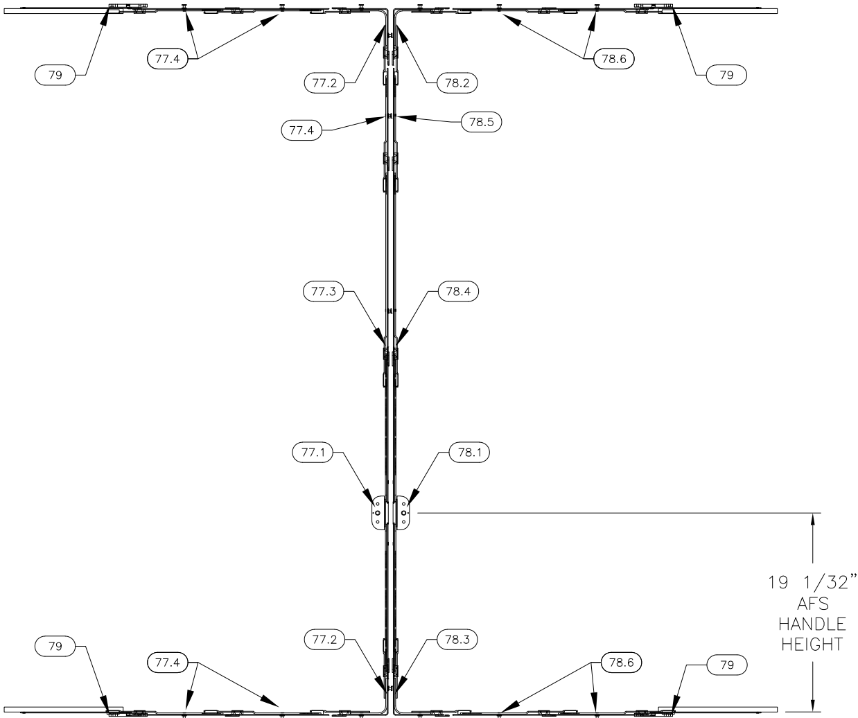
DOUBLE CASEMENT HARDWARE LAYOUT
