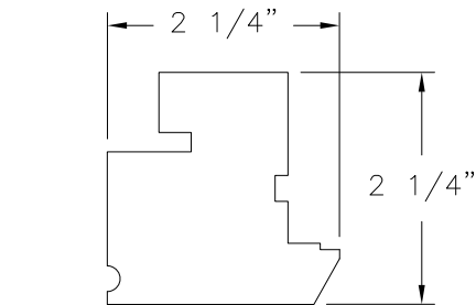
⑫ STILE (JAMB) MAHOGANY WOOD
