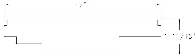
④ HEAD MAHOGANY WOOD
