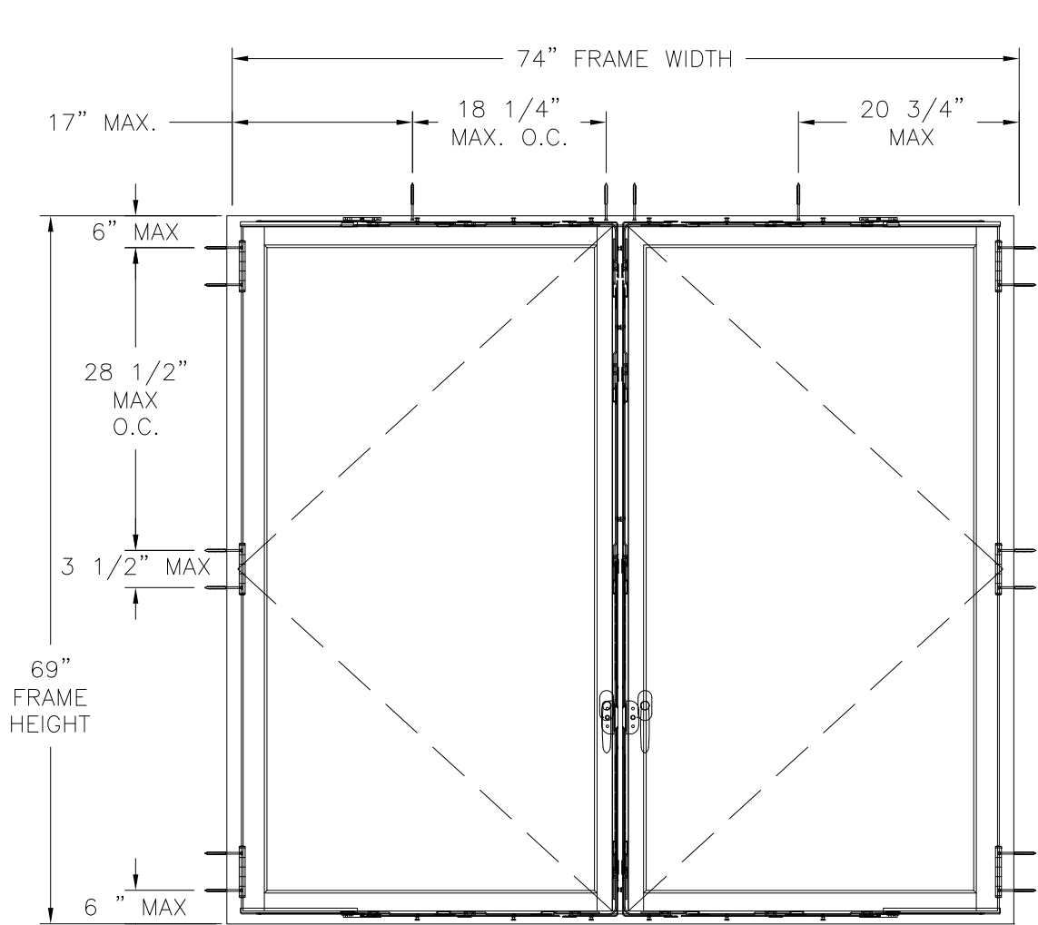
RWD WOOD INSWING - DOUBLE EXTERIOR VIEW (ANCHORS THROUGH HARDWARE & HINGES)
