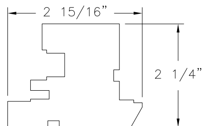
⑩ STILE (ASTRAGAL) MAHOGANY WOOD
