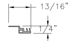
⑮ WEATHER SEAL EPDM .75" DUROMETER
