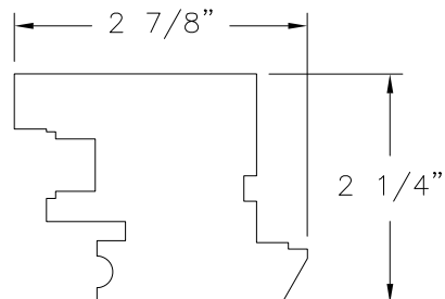
⑯ FRAME MAHOGANY WOOD
