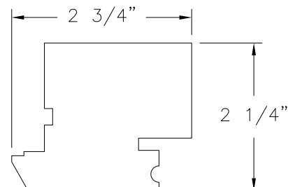
⑥ STILE (JAMB) MAHOGANY WOOD
