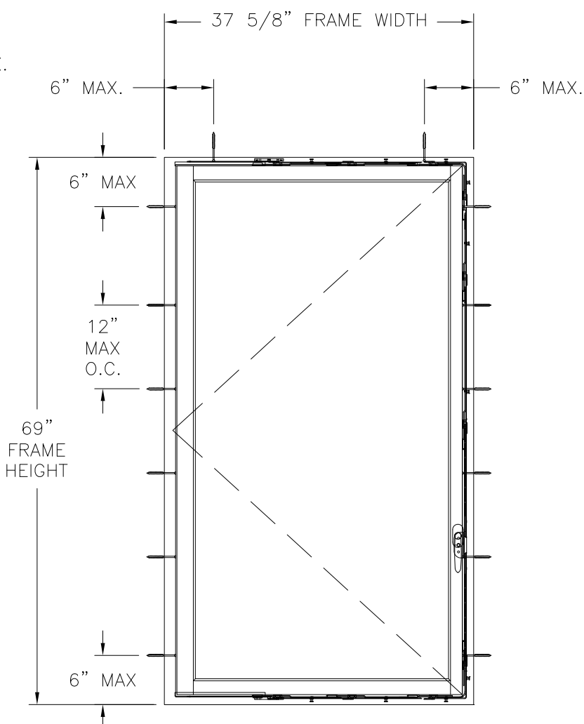
RWD WOOD INSWING - SINGLE EXTERIOR VIEW (ANCHORS THROUGH FRAME)
