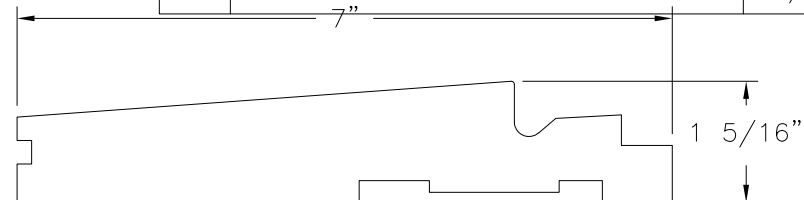
③ SILL MAHOGANY WOOD
