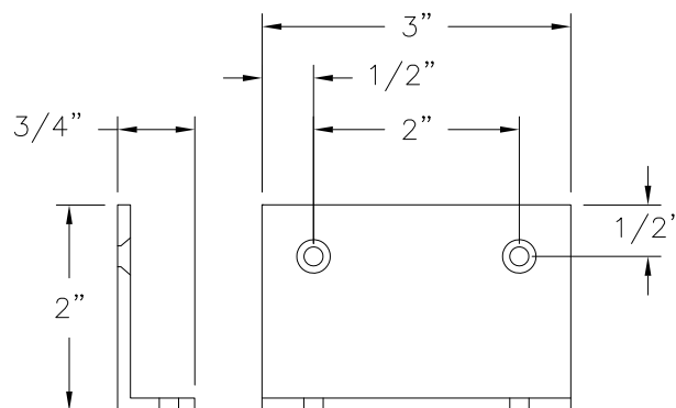
⑰ INSTALLATION ANGLE ALUMINUM 6063-T5 .125 " THICK
