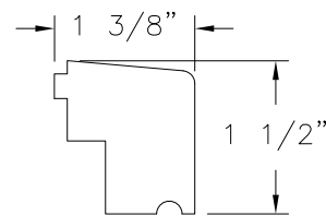
⑤ NOSING MAHOGANY WOOD
