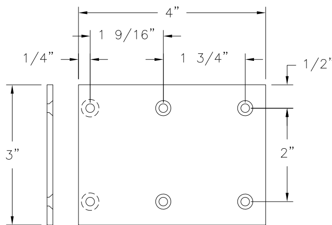
⑱ INSTALLATION BRACKET ALUMINUM 6063-T5 .125 " THICK
