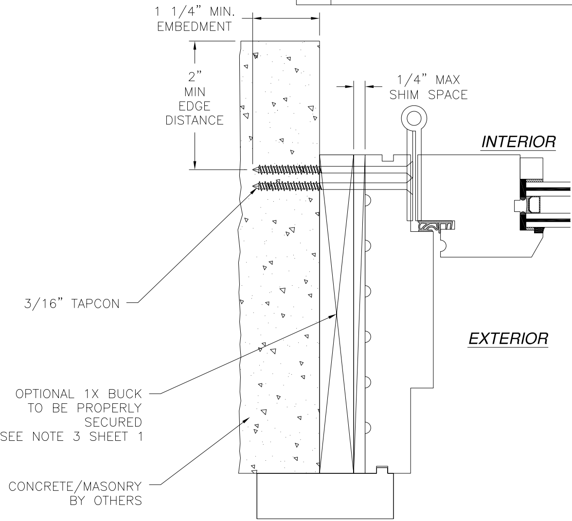
JAMB INSTALLATION DETAIL CONCRETE/MASONRY INSTALLATION
