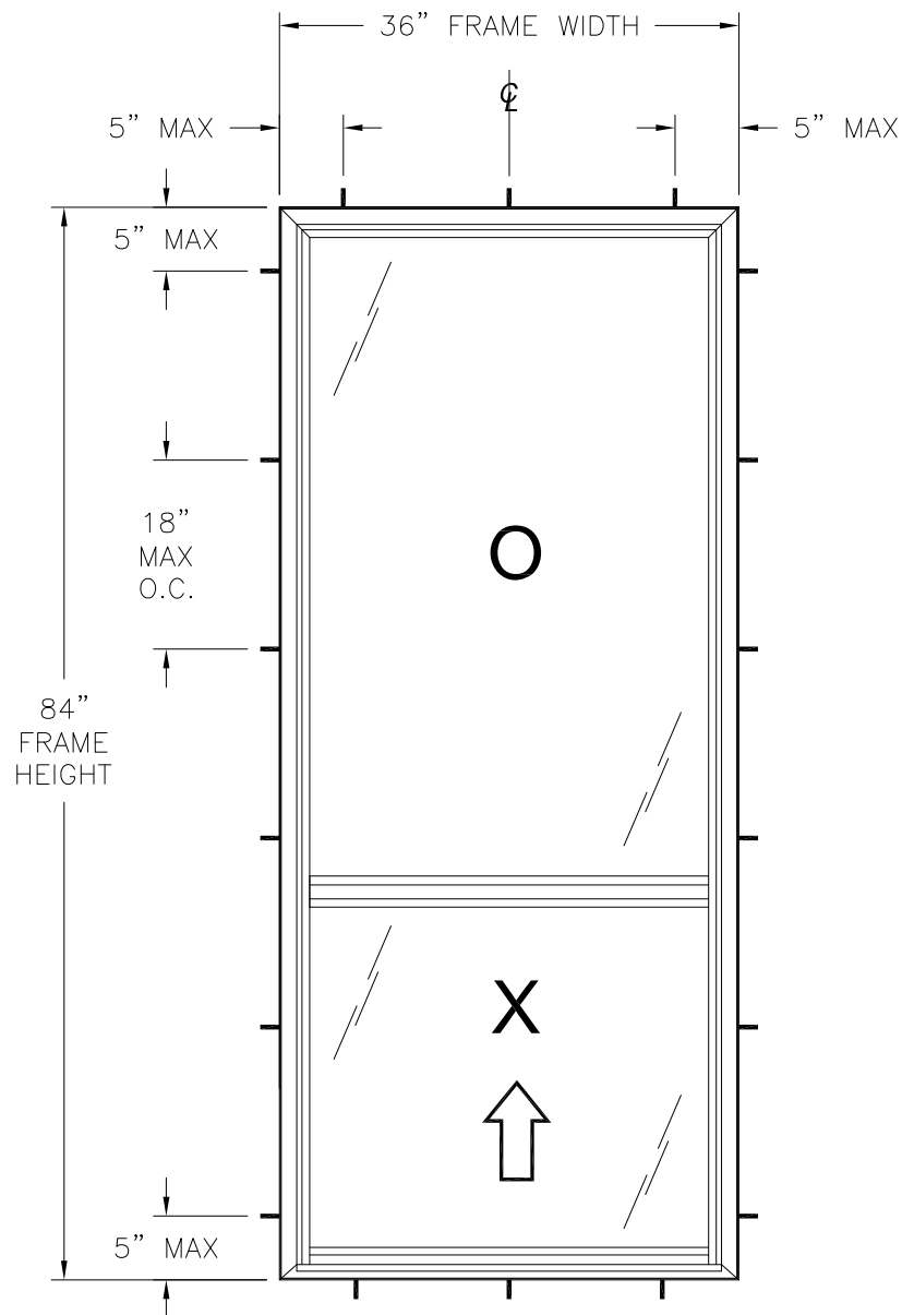
SERIES 220 SINGLE HUNG WINDOW EXTERIOR VIEW FRAME INSTALLATION
