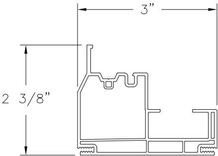
JAMB (CH9203) EXTRUDED RIGID PVC
