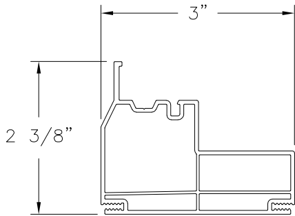
HEAD (CH9203) EXTRUDED RIGID PVC
