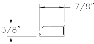
LOCK RAIL/STILE REINFORCEMENT (731-A) ALUMINUM 6063-T5
