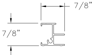
MEETING RAIL REINFORCEMENT (200A) ALUMINUM 6005-T5
