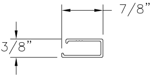
LOCK RAIL/STILE REINFORCEMENT (731-A) ALUMINUM 6063-T5
