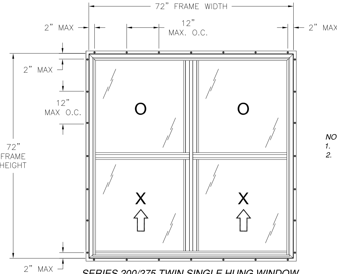
SERIES 200/275 TWIN SINGLE HUNG WINDOW EXTERIOR VIEW FIN INSTALLATION
