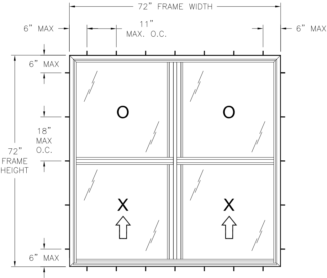
SERIES 200/275 TWIN SINGLE HUNG WINDOW EXTERIOR VIEW FRAME INSTALLATION
