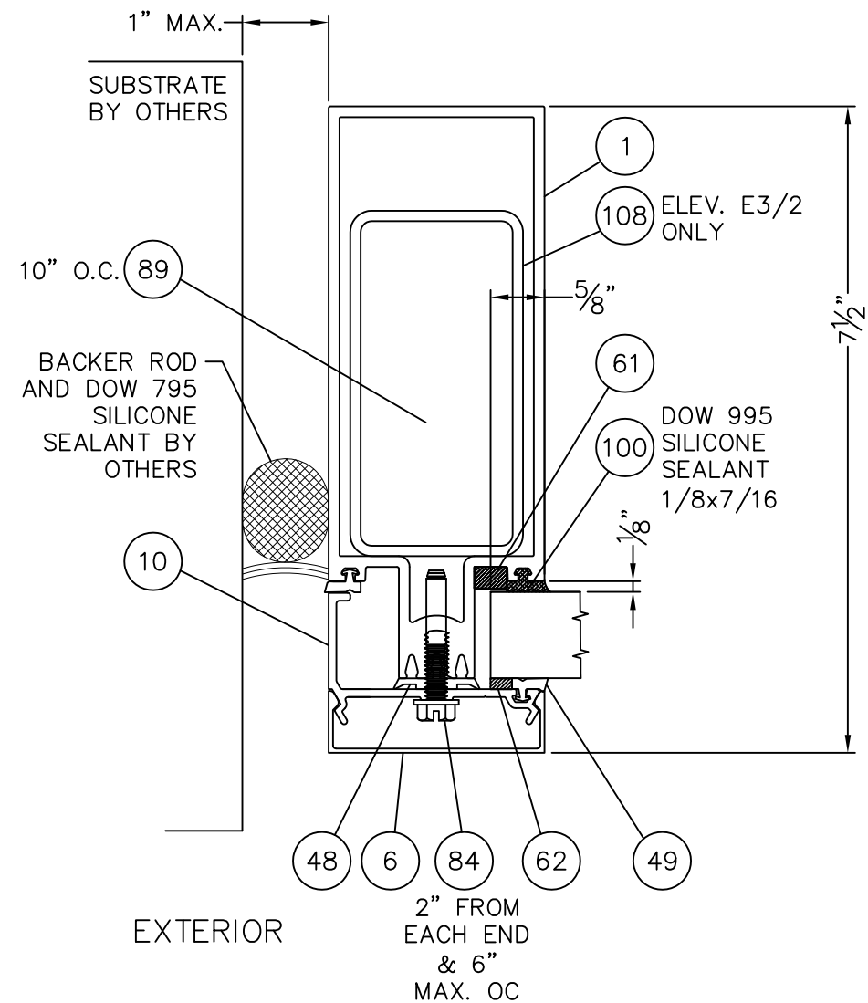
3 JAMB DETAIL SINGLE-SPAN
