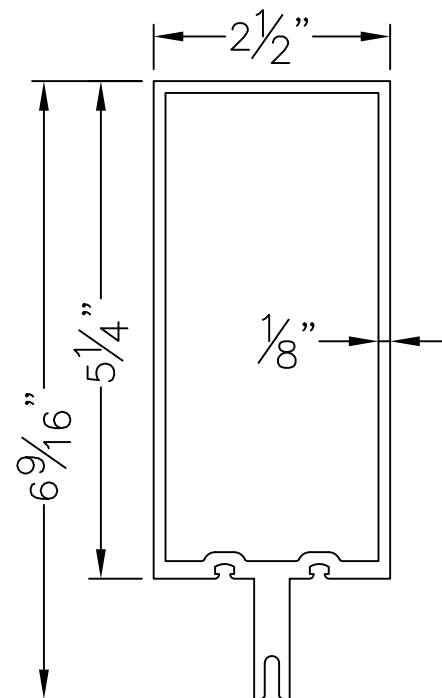
ITEM 4 – E5TB108B CURTAINWALL TUBE
