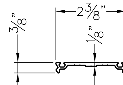
ITEM 8–M4TB224 PRESSUE PLATE (1")
