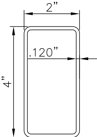
ITEM 108 P6600 2"x4"x .120 A36 STEEL TUBE
