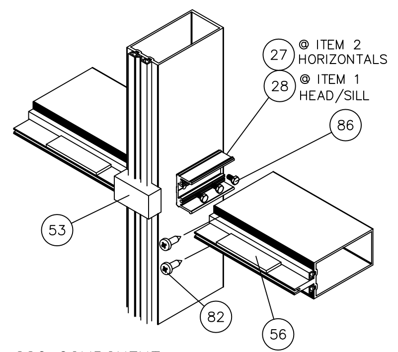
SSG COMPONENT ASSEMBLY ILLUSTRATION
