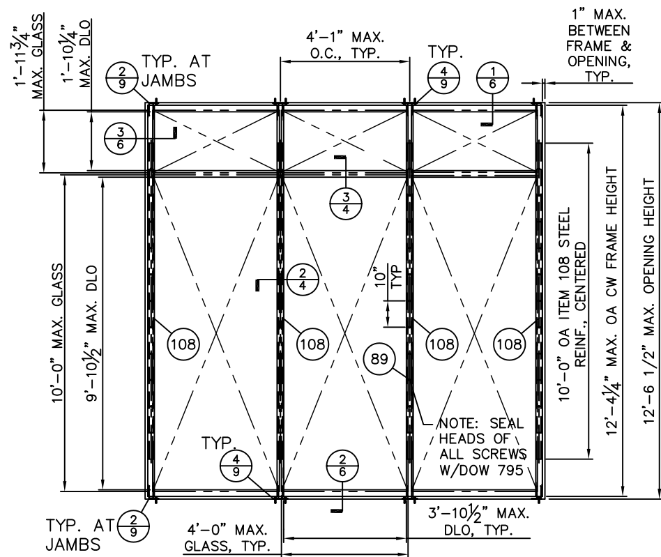
E3 2 SINGLE-SPAN ELEVATION SEE DP CHART, TABLE C
