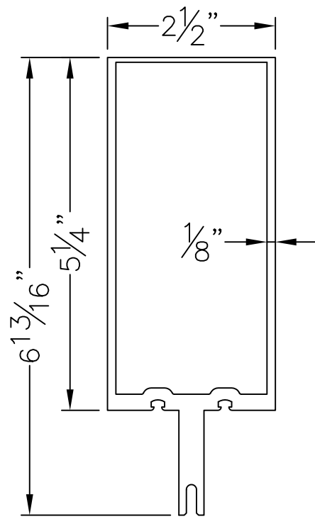
ITEM 2 – E5TB252FS CURTAINWALL TUBE
