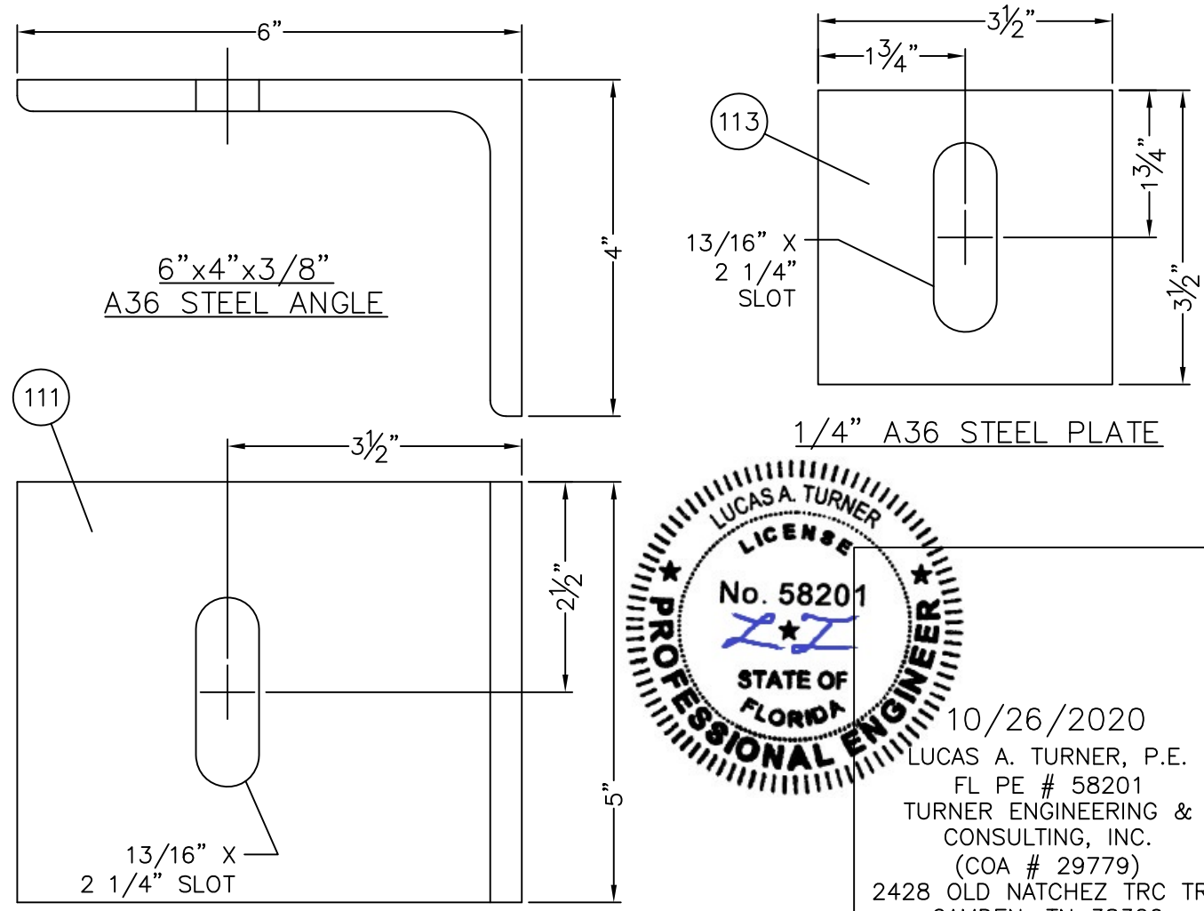
STEEL ANCHOR PARTS BY OTHERS
