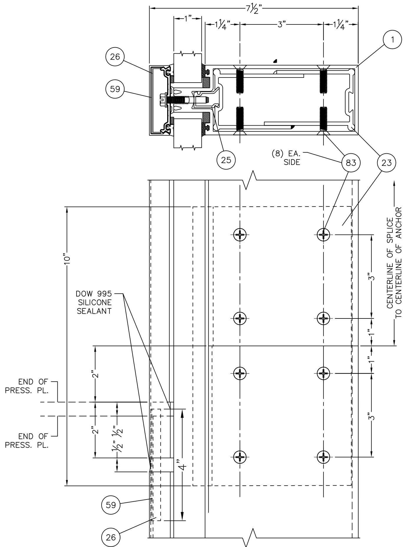
1 8 TYPICAL MULL SPLICE DETAIL
