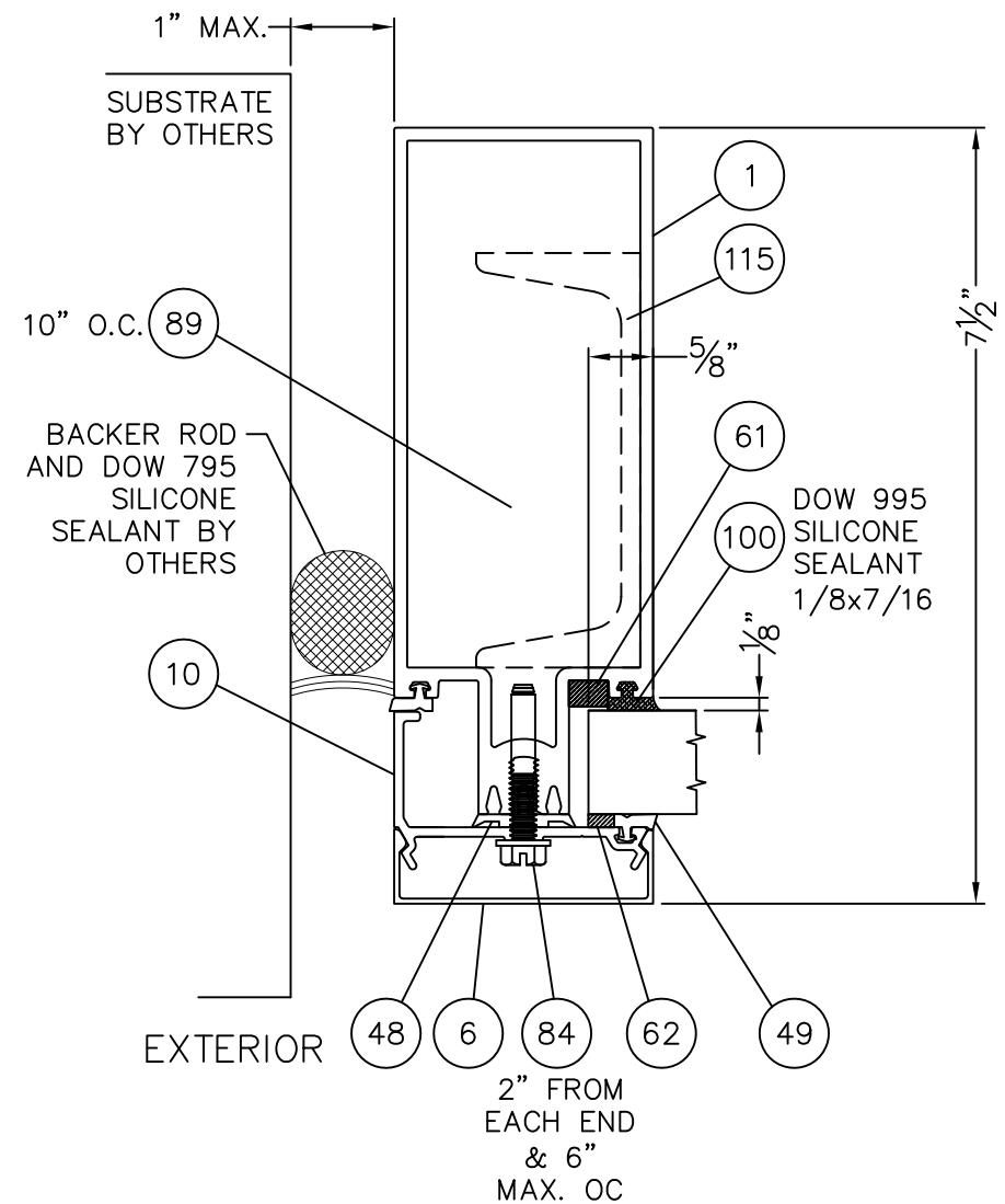
3 JAMB DETAIL TWIN-SPAN
