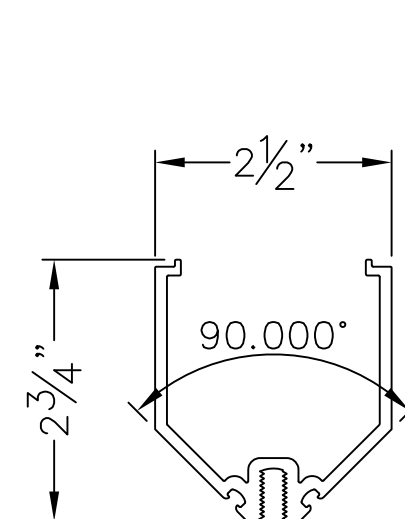
ITEM 5 – E5TB67FS OUTSIDE CORNER BUTT GLAZED CURTAINWALL ADAPTOR
