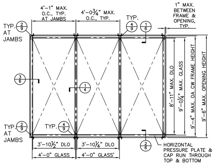
E2 2 SINGLE-SPAN ELEVATION SEE DP CHART, TABLE B
