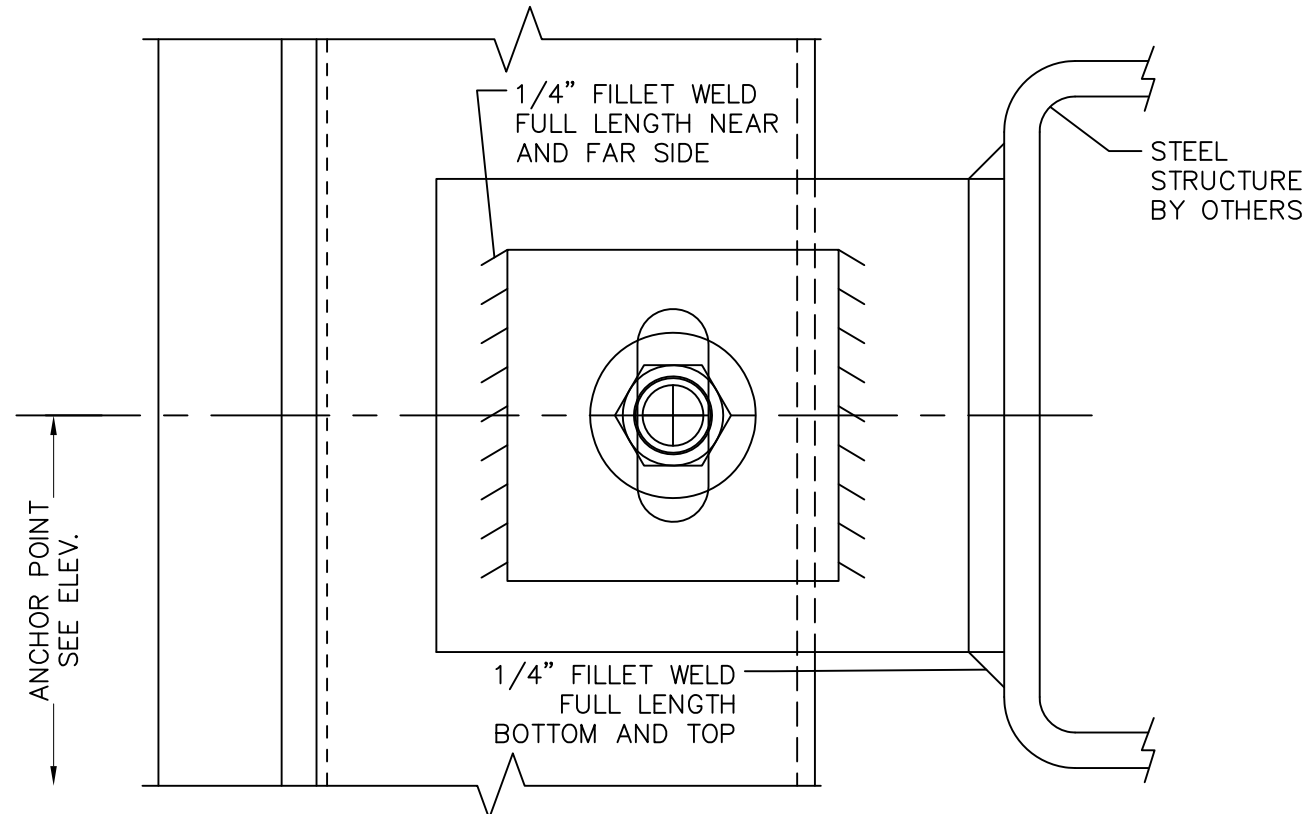
1 10 STRUCTURAL GLAZED MULL ANCHOR DETAIL SIMILAR AT CORNER MULL WITH FORMED ANGLES
