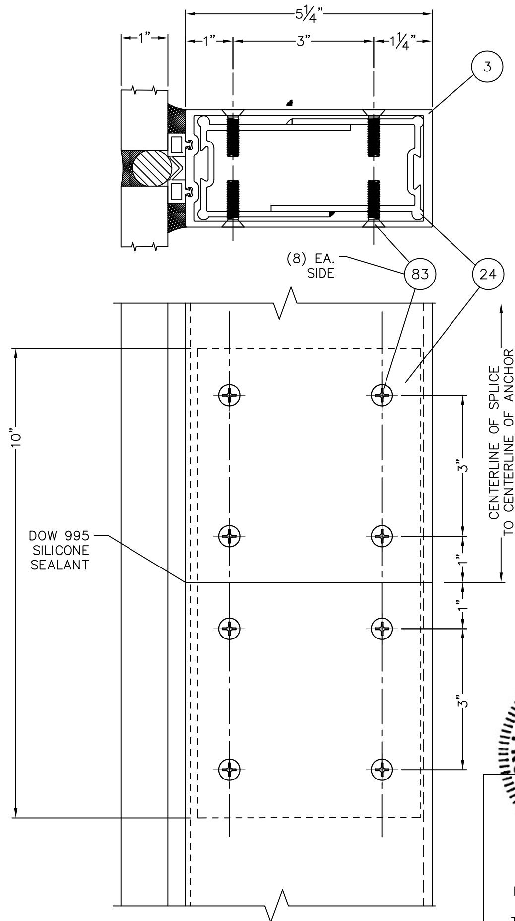
2 8 STRUCTURAL GLAZED MULL SPLICE DETAIL
