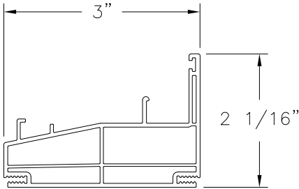
SILL (CH9202) EXTRUDED RIGID PVC
