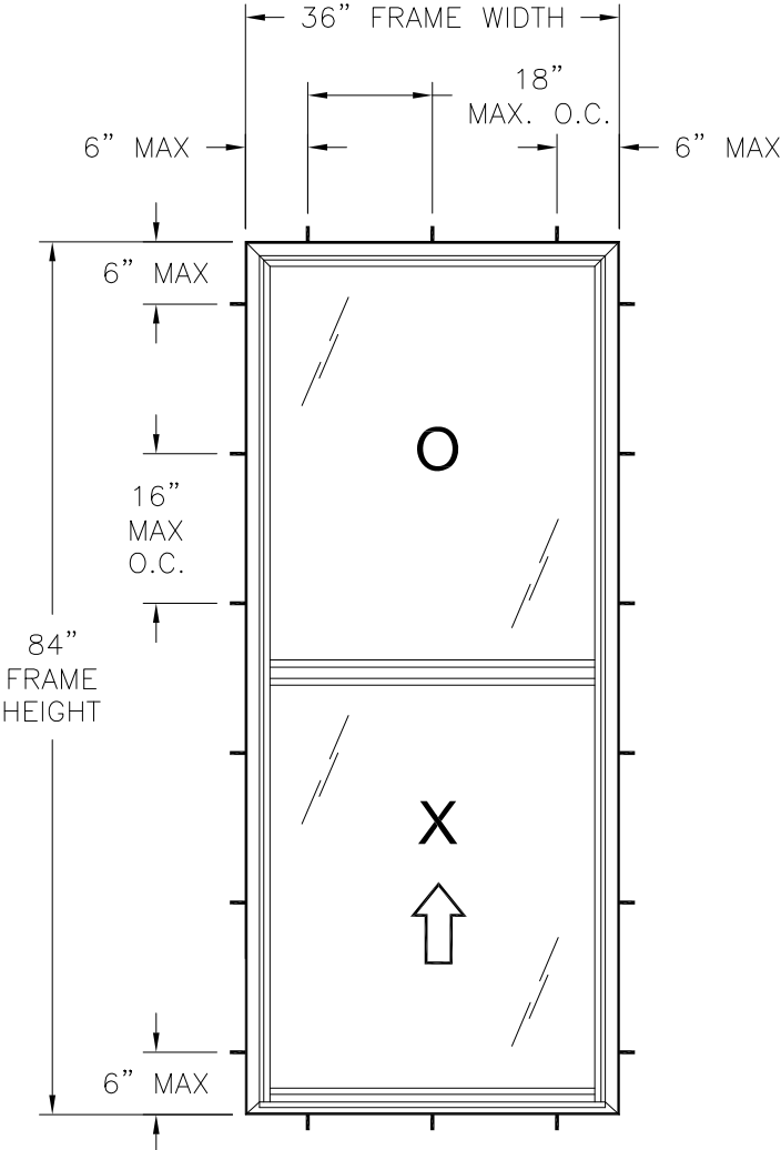
SERIES 200/275 SINGLE HUNG WINDOW EXTERIOR VIEW FRAME INSTALLATION
