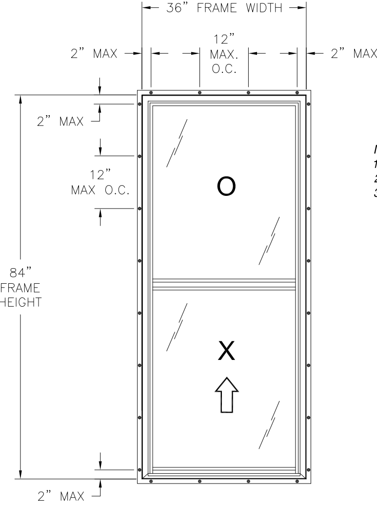
SERIES 200/275 SINGLE HUNG WINDOW EXTERIOR VIEW FIN INSTALLATION
