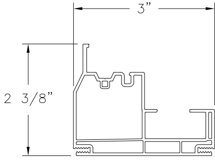
HEAD AND JAMB (CH9203) EXTRUDED RIGID PVC
