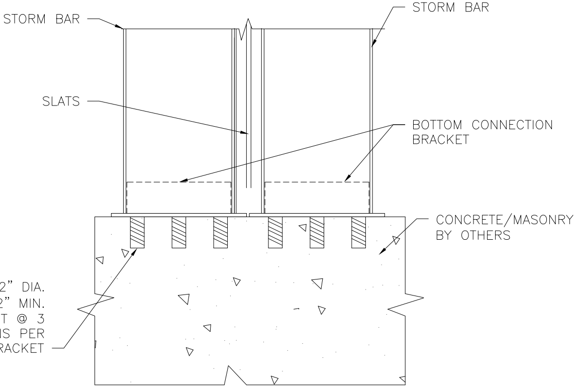
C 5 VERTICAL CROSS SECTION (OPTIONAL) BOTTOM STORM BAR INSTALLATION
