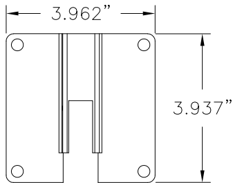
28 IDLE BRACKET
