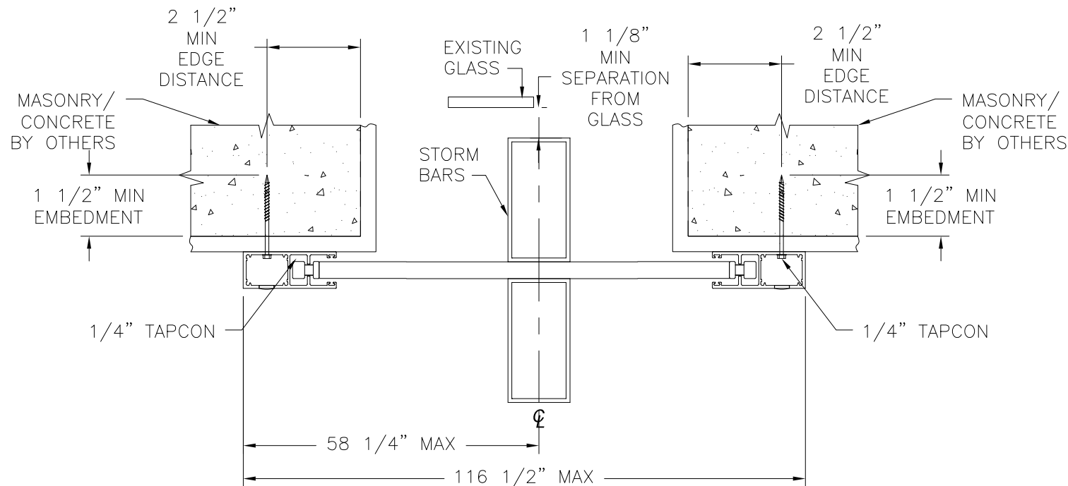
B 3 HORIZONTAL CROSS SECTION UNITS WITH STORM BARS 60" WIDE UP TO 116 1/2" WIDE
