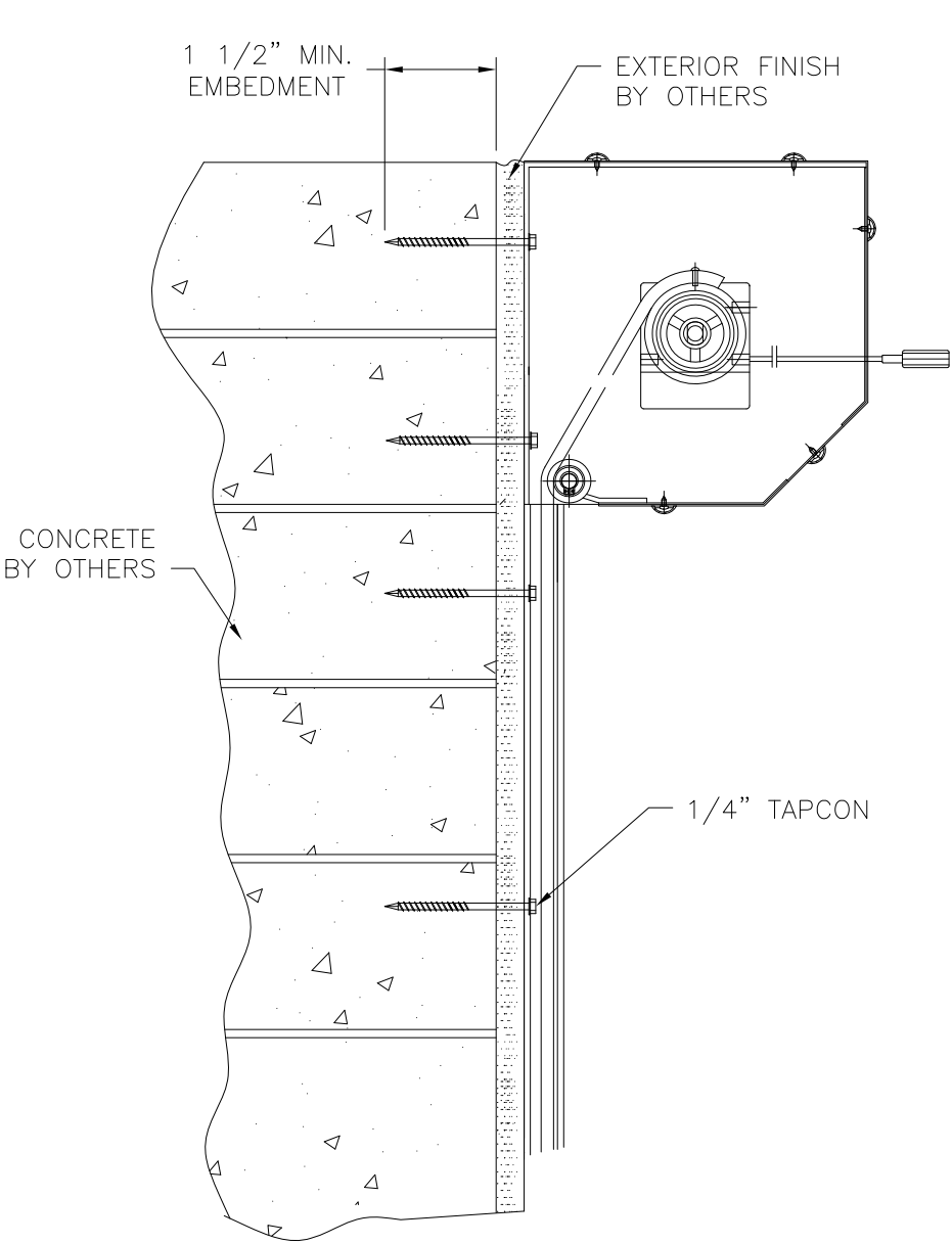
A 4 VERTICAL CROSS SECTION CONCRETE INSTALLATION
