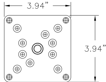
6 MOTOR BRACKET
