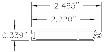
10 56 MM END RAIL 6063-T5 ALUMINUM .039" THICK
