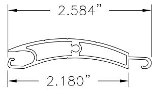
8 55 MM SLAT 6063-T5 ALUMINUM .053" THICK
