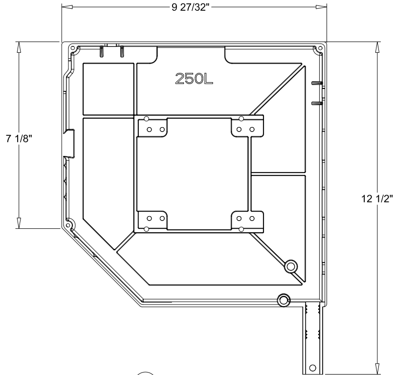
1 250 MM HOOD
