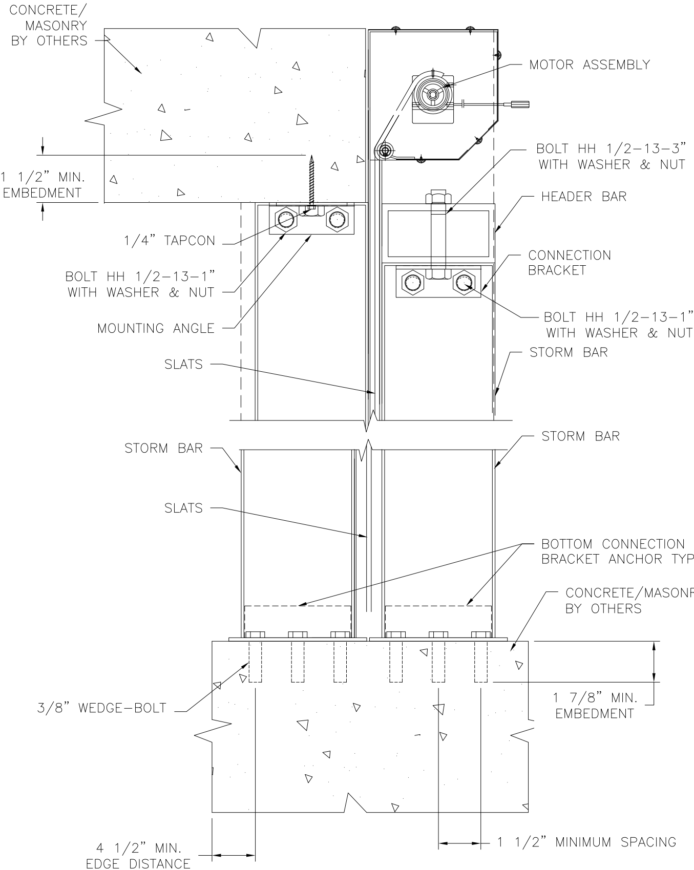
C 5 VERTICAL CROSS SECTION STORM BAR INSTALLATION
