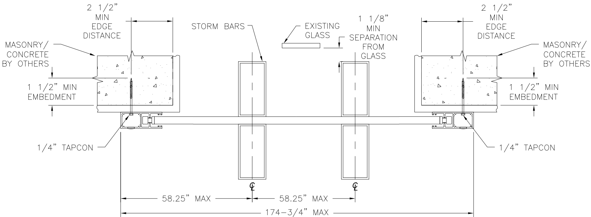
B 3 HORIZONTAL CROSS SECTION UNITS WITH STORM BARS 117" WIDE UP TO 174 3/4" WIDE
