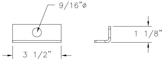
24 MOUNTING ANGLE 14 GA. (0.078" THICK) GALVANIZED STEEL
