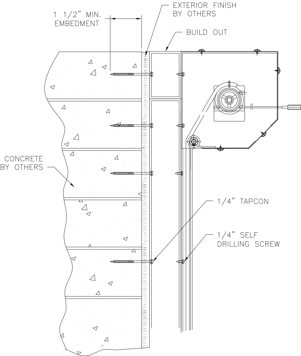
A 4 VERTICAL CROSS SECTION (BUILD-OUT) CONCRETE INSTALLATION
