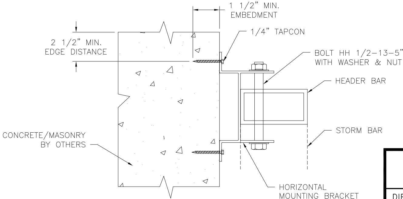
D/6 VERTICAL CROSS SECTION HEAD BAR INSTALLATION
