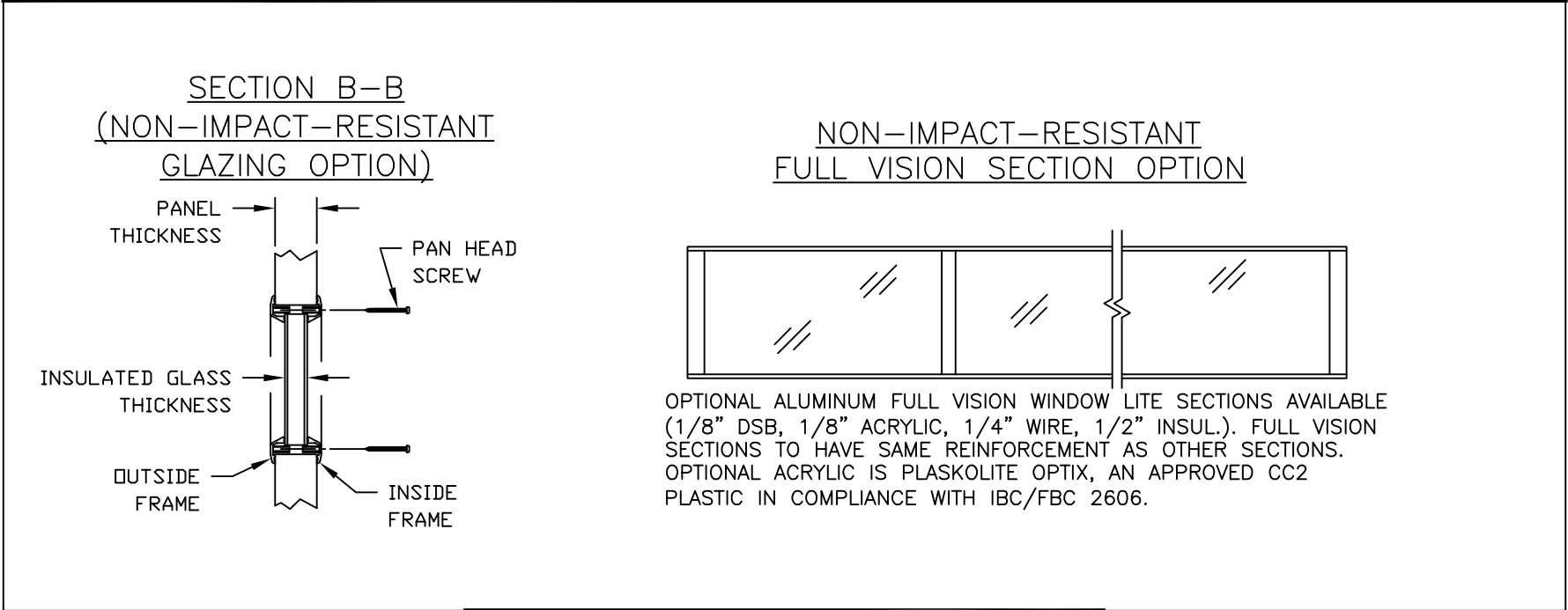
STANDARD ASSEMBLY DETAILS DRAWING 104861-B
