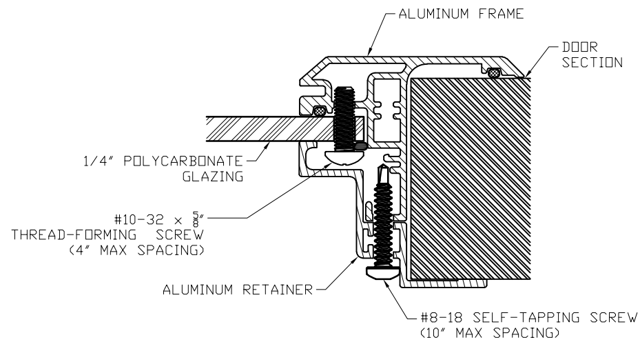
IMPACT-RESISTANT ASSEMBLY DETAILS DRAWING 104039-A
