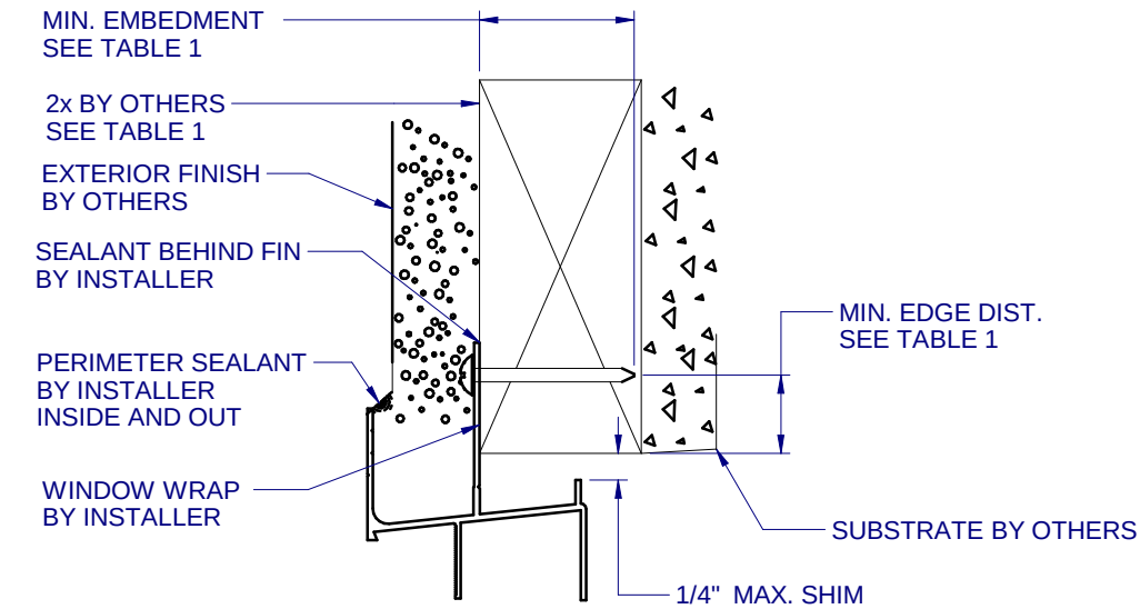
TYPICAL HEAD ANCHORAGE
