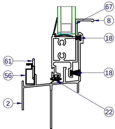
SECTION VIEW A-A
