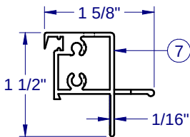
SASH TOP RAIL H-1072
