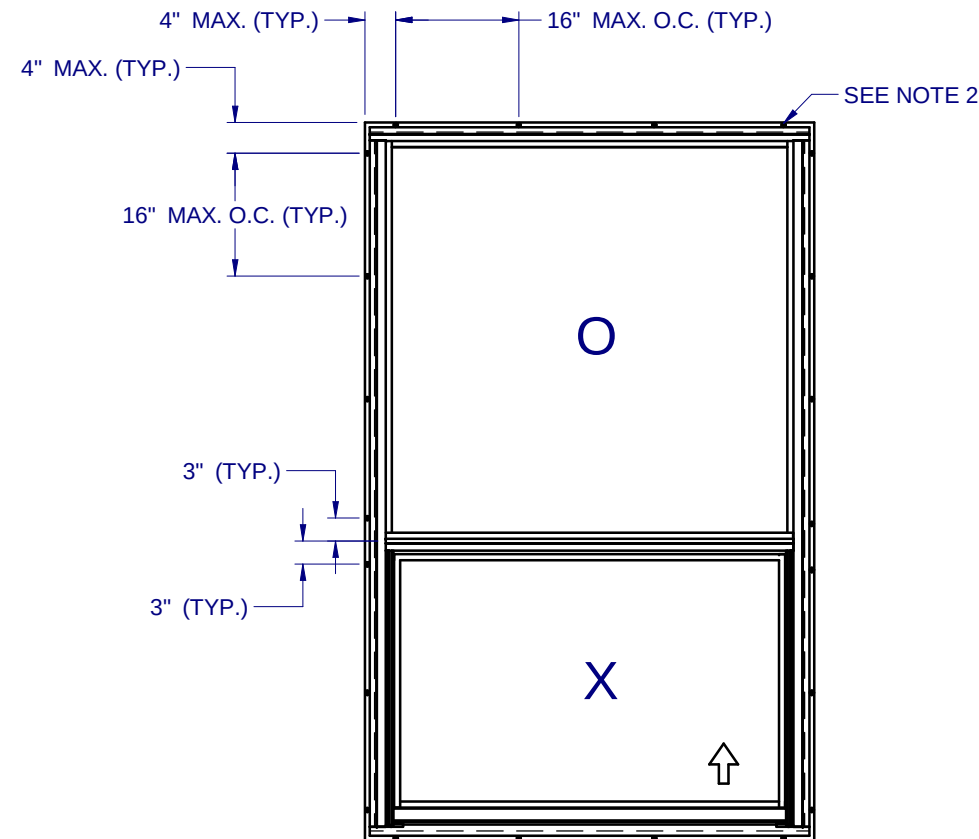
ANCHOR LAYOUT - (FIN) THRU FIN (WOOD)
