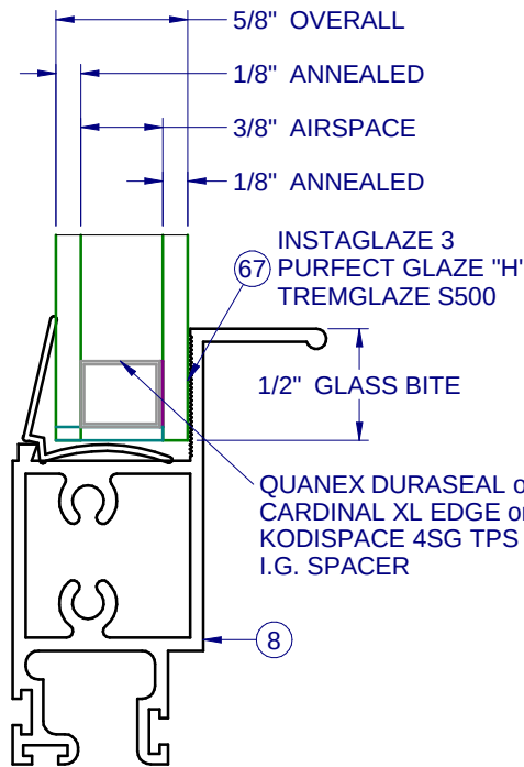
GLASS TYPE A 1:1
