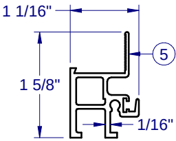
FIXED RAIL H-1563
