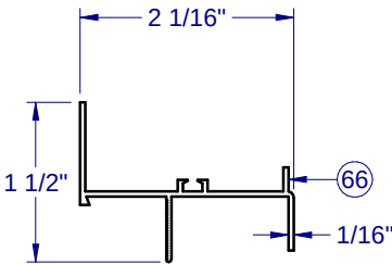
FLANGE HEAD, ARCHTOP S-1114 (USED WITH S-1126)
