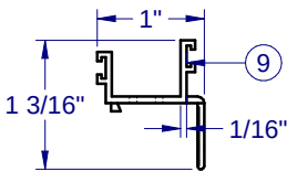
SASH SIDE RAIL S-1073
