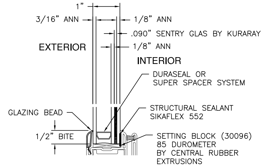
GLAZING DETAIL
