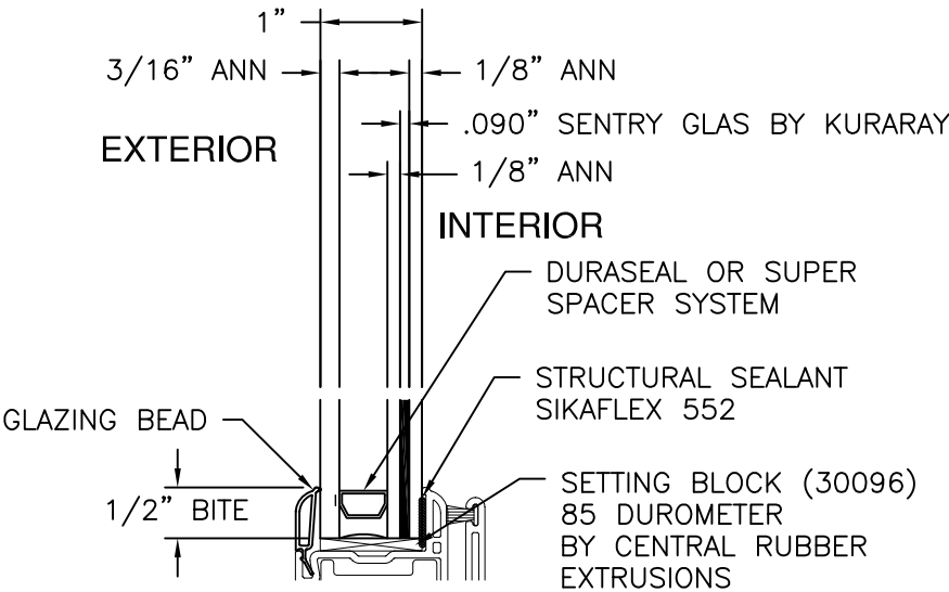
GLAZING DETAIL
