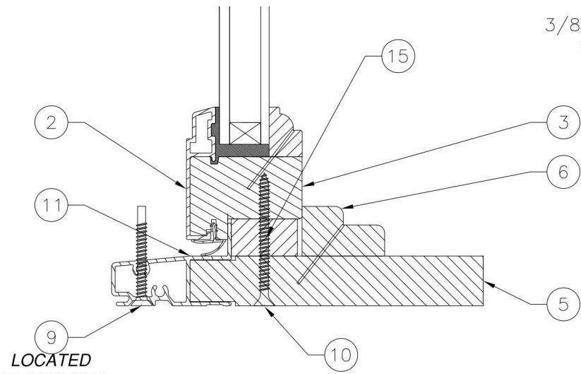
VERTICAL SECTION
