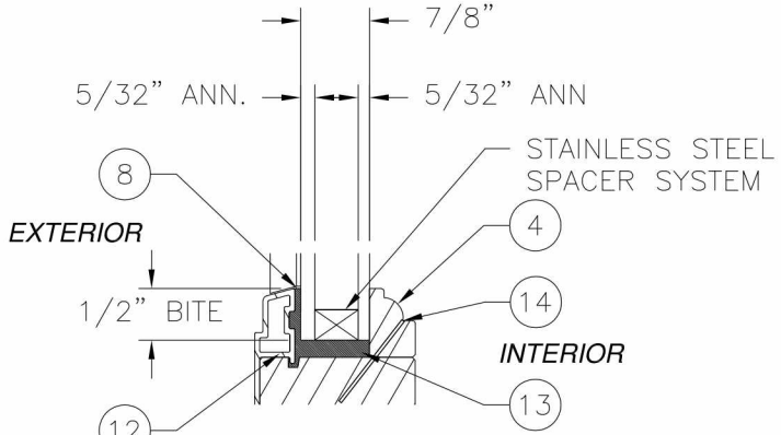
GLAZING DETAIL
