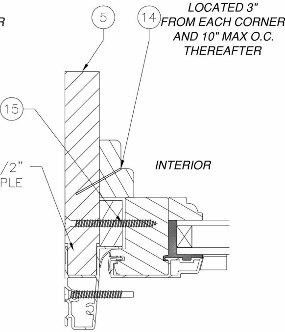
EXTERIOR HORIZONTAL SECTION
