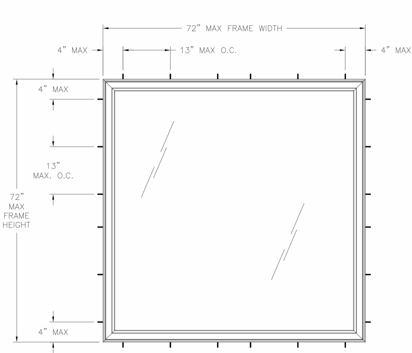
400 CLAD CASEMENT PICTURE WINDOW EXTERIOR VIEW FRAME INSTALLATION
