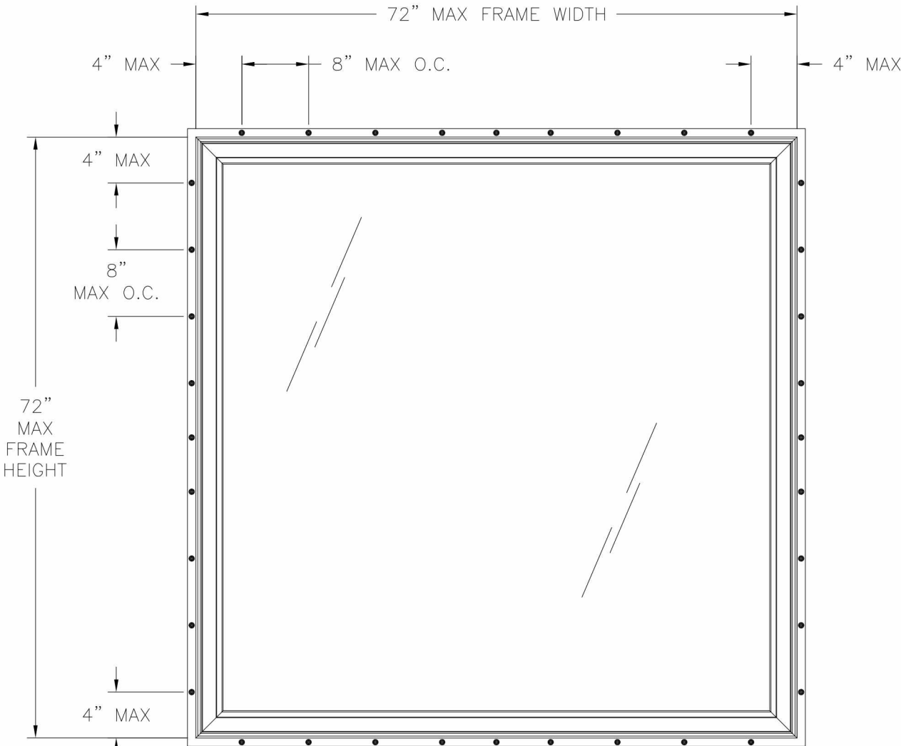
400 CLAD CASEMENT PICTURE WINDOW EXTERIOR VIEW FIN INSTALLATION
