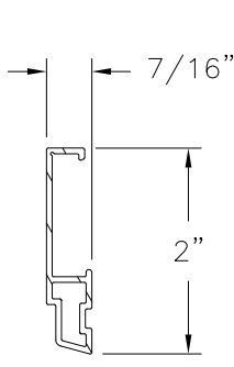
2 SASH CLAD ALUMINUM 6063-T5 .069" THICK
