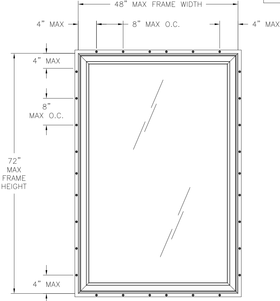
400 CLAD CASEMENT PICTURE WINDOW EXTERIOR VIEW FIN INSTALLATION
