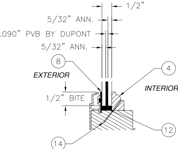
GLAZING DETAIL A
