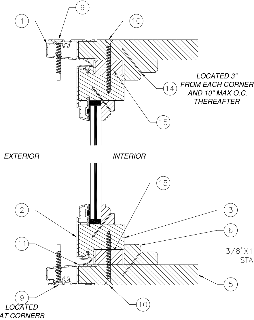
VERTICAL SECTION
