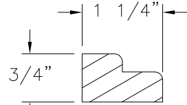
6 INTERIOR STOP PINE
