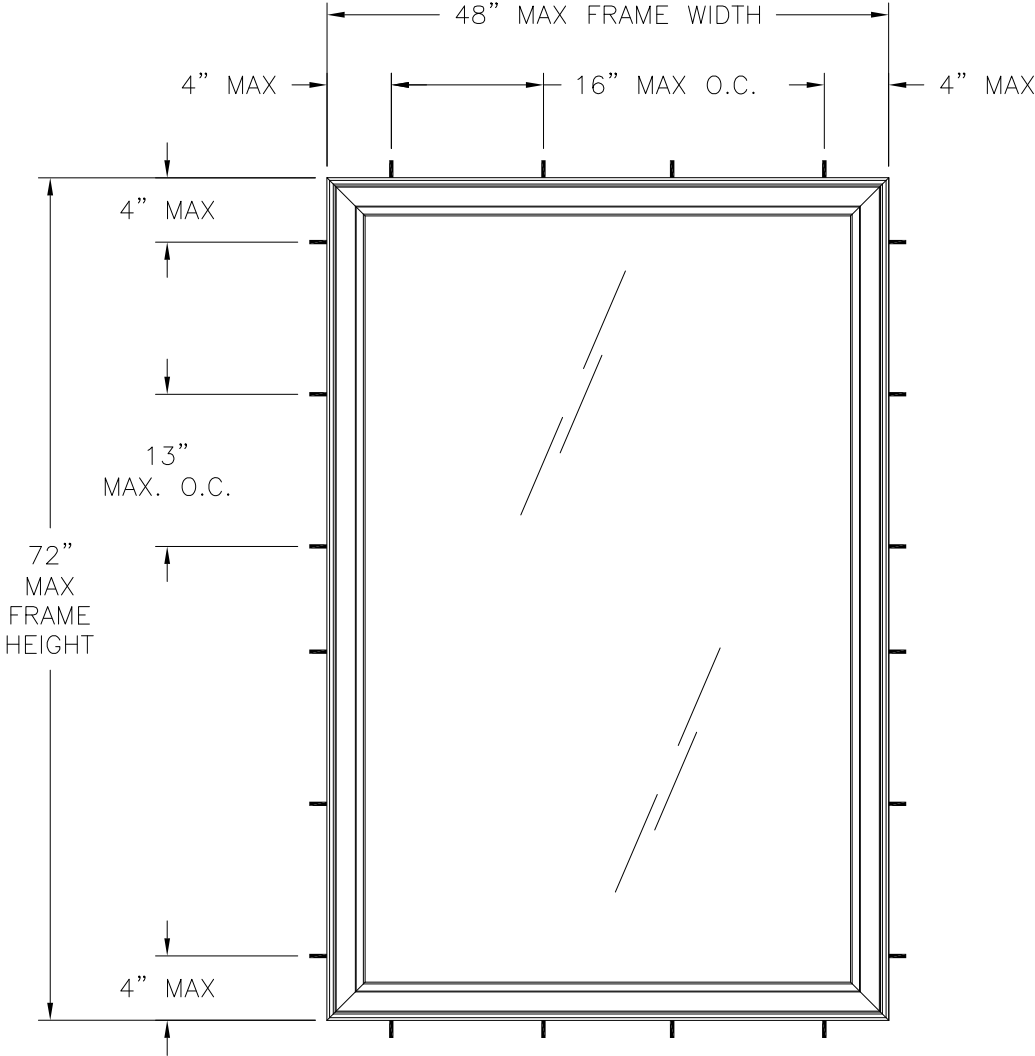
400 CLAD CASEMENT PICTURE WINDOW EXTERIOR VIEW FRAME INSTALLATION
