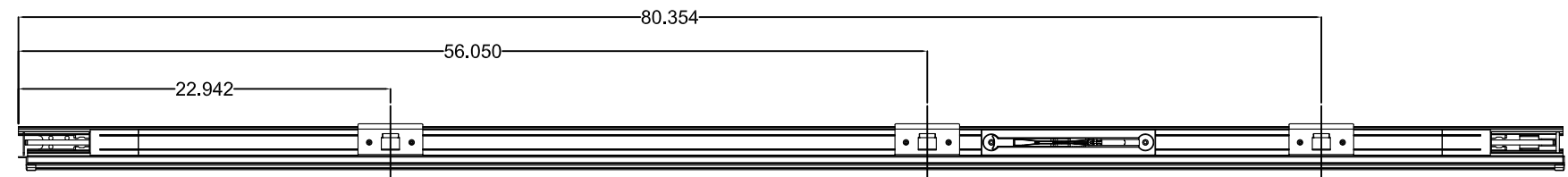
HARDWARE LOCATIONS
