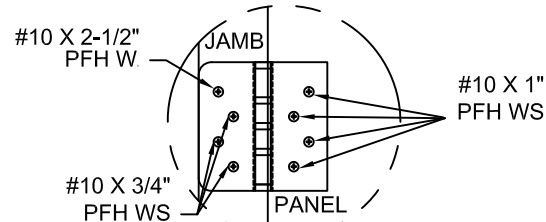
HINGE DETAIL
