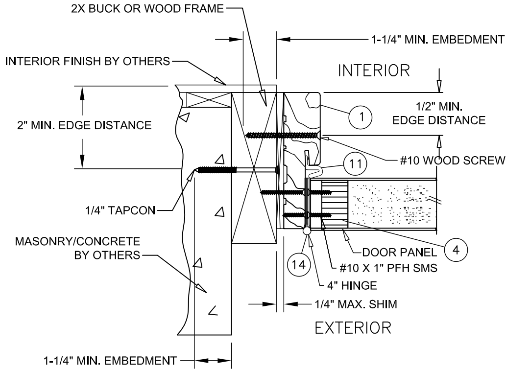
H 6 HORIZONTAL CROSS SECTION OUTSWING SHOWN-INSWING SIMILAR 2X BUCK OR WOOD FRAME OCNCTRCTION
