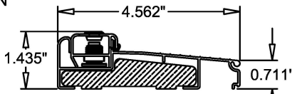
36 INSWING THRESHOLD ALUMINUM / WOOD BY ENDURA ZAILAA4565
