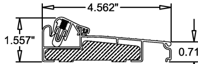
34 INSWING THRESHOLD ALUMINUM / WOOD BY ENDURA ZA4565
