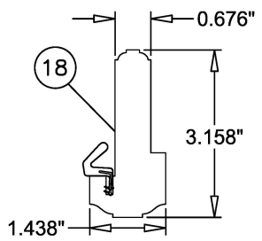
ASTRAGAL SECTION
