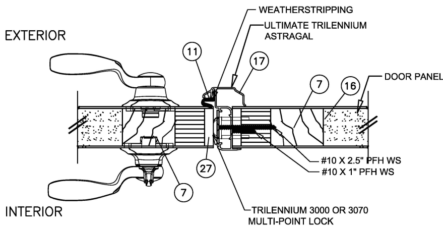
F 3 ASTRAGAL SECTION INSWING SHOWN-OUTSWING SIMILAR
