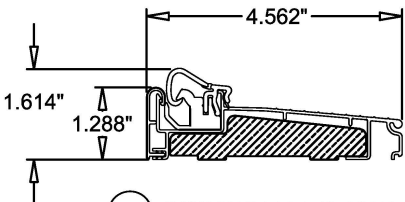
3 INSWING THRESHOLD ALUMINUM / WOOD BY ENDURA ZA4565
