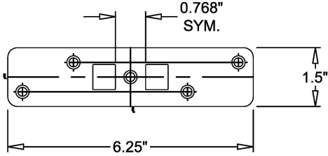
23 3500 / 3020 STRIKE PLATE STEEL
