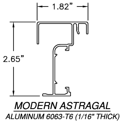
ASTRAGAL ALUMINUM 6063-T6 (1/16" THICK)
