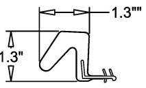
11 WEATHERSTRIPPING PE-650 FOAM
