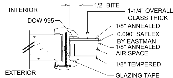
RSL GLAZING DETAIL ALUMINUM SPACER
