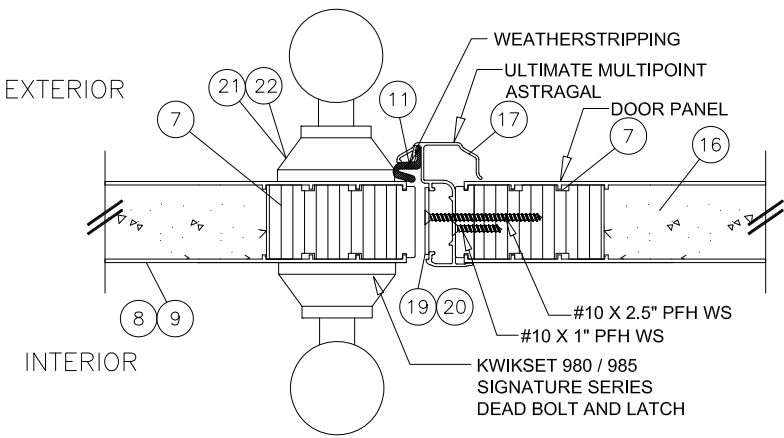
E ASTRAGAL SECTION 2 INSWING SHOWN-OUTSWING SIMILAR
