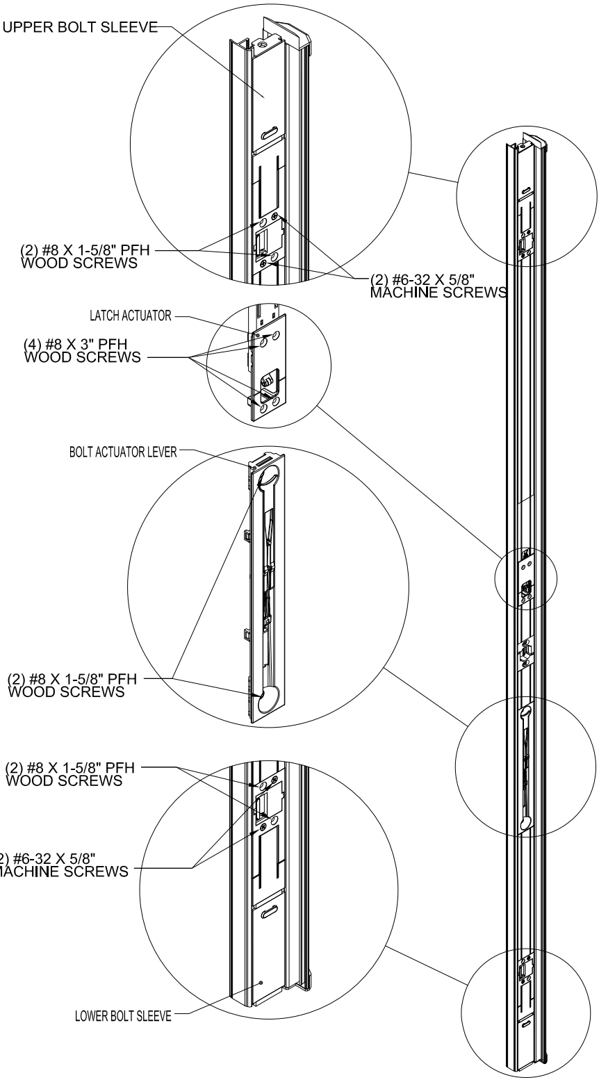
ULTIMATE MULTIPOINT ASTRAGAL
