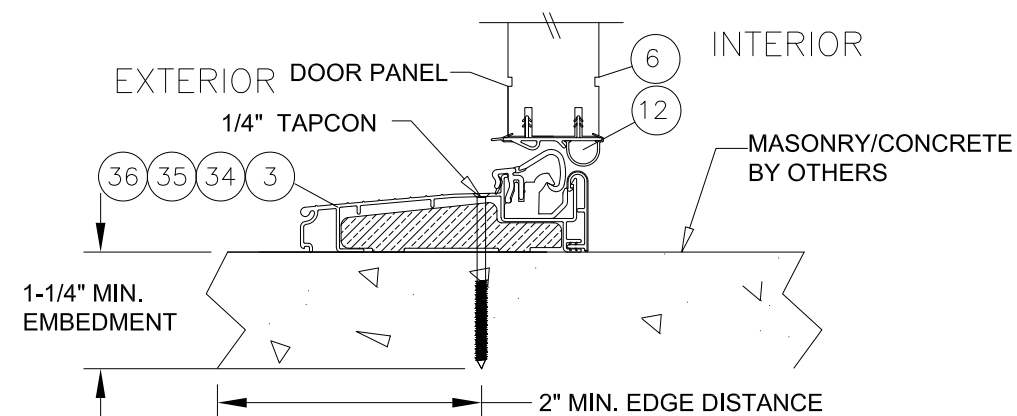
C 6 VERTICAL CROSS SECTION IN-SWING "Z" SERIES SILL (ZACL4565)
