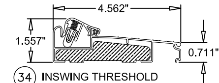
34 INSWING THRESHOLD ALUMINUM / WOOD BY ENDURA ZACLA4565
