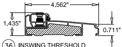
36 INSWING THRESHOLD ALUMINUM / WOOD BY ENDURA ZAILAA4565
