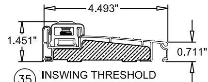
35 INSWING THRESHOLD ALUMINUM / WOOD BY ENDURA ZAIL4565
