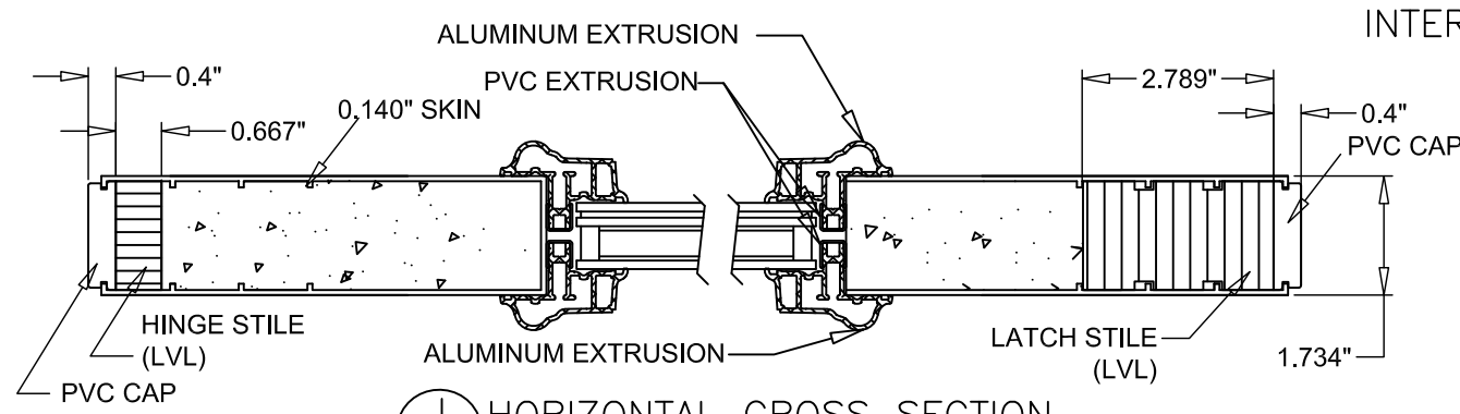
J 5 HORIZONTAL CROSS SECTION ODL SEVERE WEATHER GLAZING INSERT OPTION
