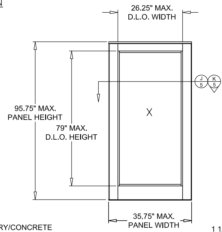
PLASTPRO GLAZED INSERT FIBERGLASS
