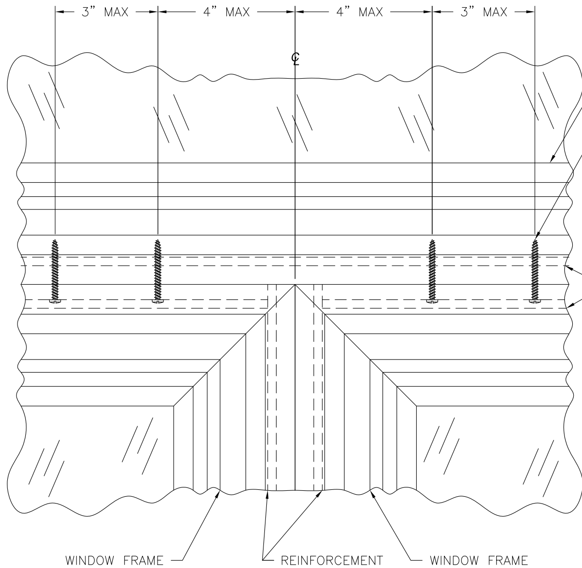
TRANSOM/WINDOW CONNECTION DETAIL A SEE DETAIL D SHEET 7 FOR FRAME TO REINFORCEMENT INSTALLATION
